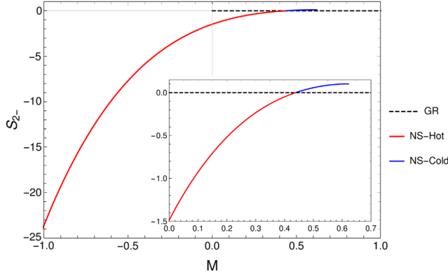
FIG. 1. Solutions space of non-Schwarzschild BHs. Red line indicates non-Schwarzschild black holes which are hotter than Schwarzschild black holes, blue line indicates colder black holes which are instead obtained for S_{2-} > 0 .
