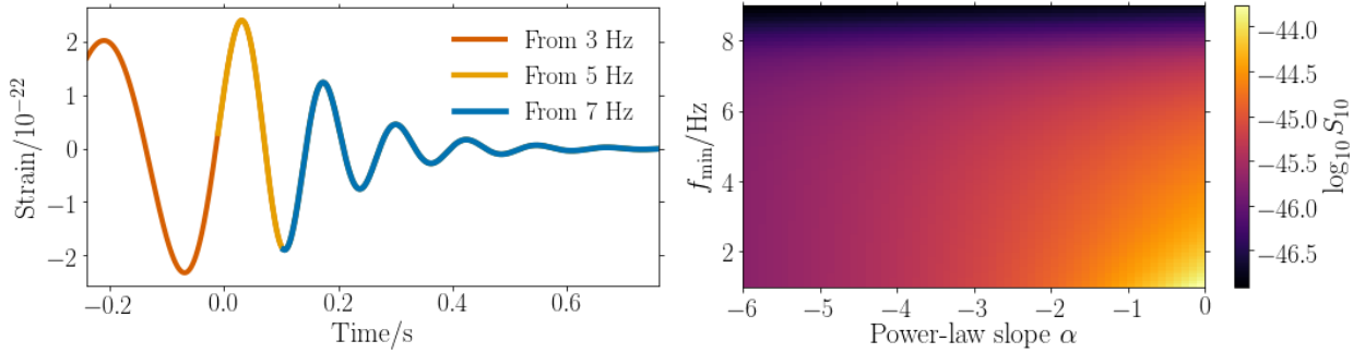
Figure 2: Left: The waveform from the final stages of inspiral, merger and ringdown of a 100M_\odot + 100M_\odot BBH at a redshift of z = 10 . Highlighted is the time evolution of the waveform from 3, 5 and 7 Hz. Right: Requirements on the low-frequency noise power spectrum S_n(f) necessary to detect an overhead, face-on 100M_\odot + 100M_\odot BBH merging at z = 10 . We assume a power-law form S_n(f) \propto f^\alpha extending down to a minimum frequency f_{\min} with the specified normalization S_{10} at f = 10 Hz.
