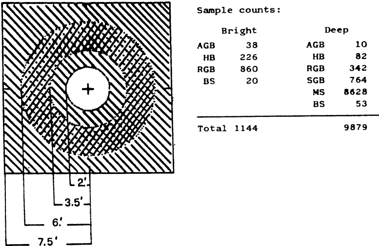
Fig. 2: Observed fields and number of stars in each individual sample.
