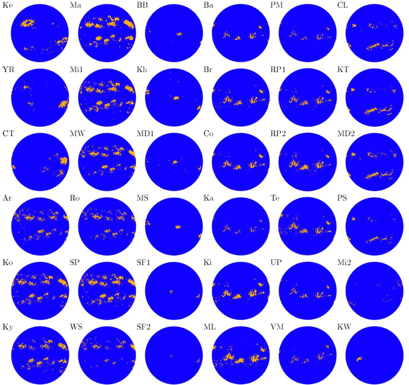
Fig. 6. Segmentation masks derived from the observations shown in Figs. 1 and 5. Plage are highlighted in yellow, while quiet Sun and network regions together form the blue background. We stress that the same threshold have been used for all datasets to identify the plage regions, which is why the different datasets seem to give rather different plage coverage depending on the employed bandwidth or central wavelength.
