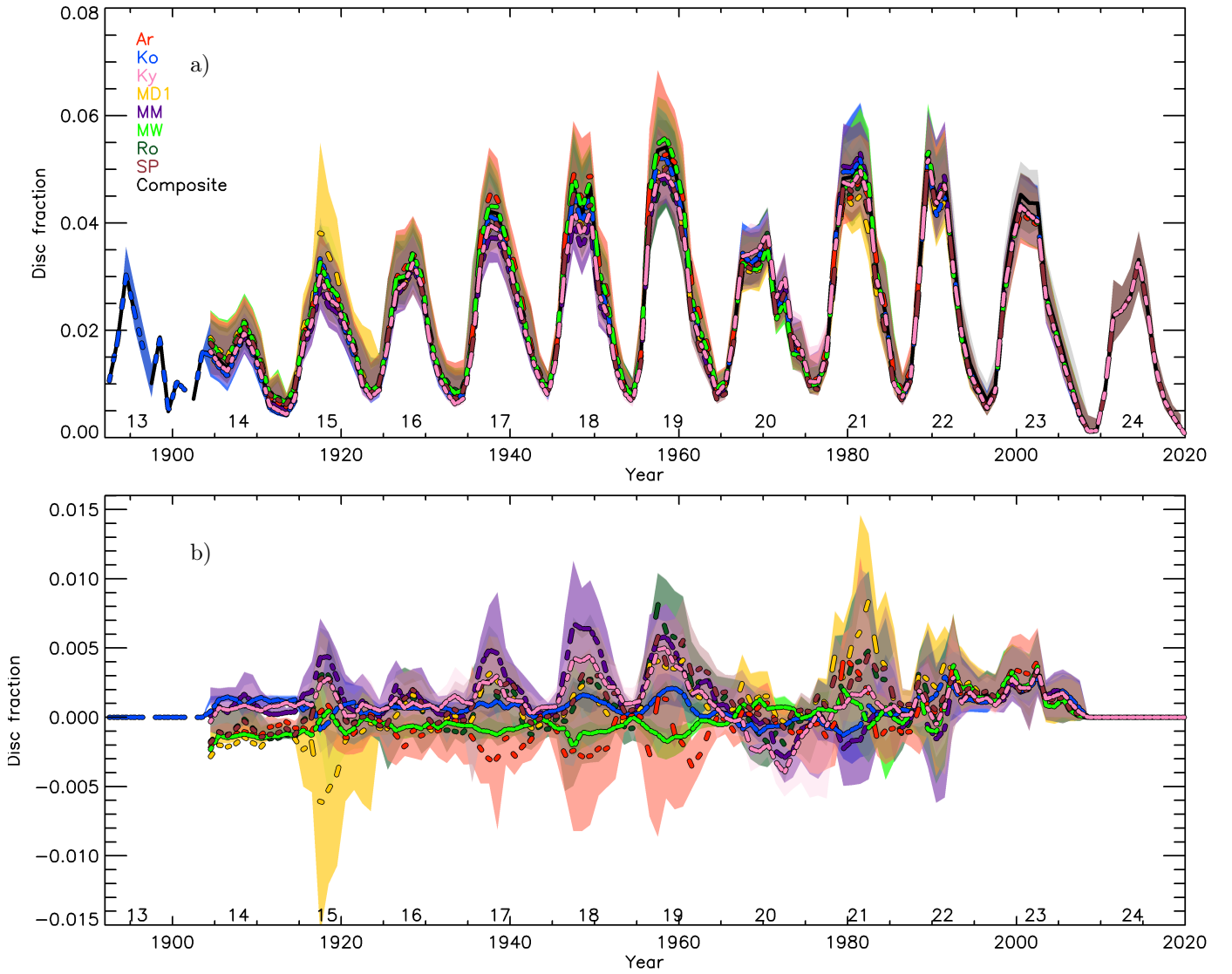
Fig. 14. Plage area composites (a) and their difference to our main composite series (b) when the historical backbone series was computed with various individual historical datasets as the backbone reference instead of using the average of the calibrated Ko and MW ones to the RP1 one. RP1 is always taken as the overall reference for all composite series. The datasets used as backbones are those from Ar (red), Ko (blue), Ky (pink), MD1 (orange), MM (purple), MW (green), Ro (dark green), and SP (brown) sites. The composite plage area series derived in this study is also displayed in black. Shown are the annual median values (lines) of the final plage area composites along with the asymmetric 1\sigma interval (shaded surfaces). The numbers below the curves denote the conventional SC numbering.
