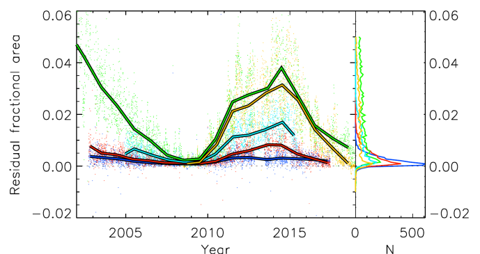
Fig. 13. Left: Difference of fractional plage area between those derived from centred and off-centred Ca II K observations as a function of time. The differences shown are for the Co-CoW (orange), MD1-MDW (green), MD1-MDV (blue), MD1-MDR (red), ML-MLW (cyan). Dots show daily values, while the solid lines show annual median values. The dotted horizontal line denotes a difference of 0. Right: Distributions of the differences.
