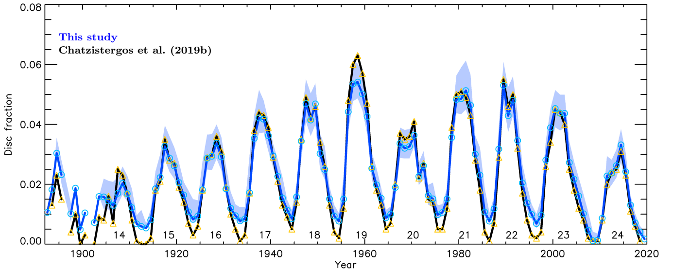
Fig. 9. Composite of plage areas in disc fraction derived in this study (blue line and open circles) along with the composite by Chatzistergos et al. (2019b, black line and open triangles). Shown are annual median values (solid lines and symbols) along with the asymmetric 1\sigma interval (shaded surfaces). The solar cycle numbers are given below the curves.
