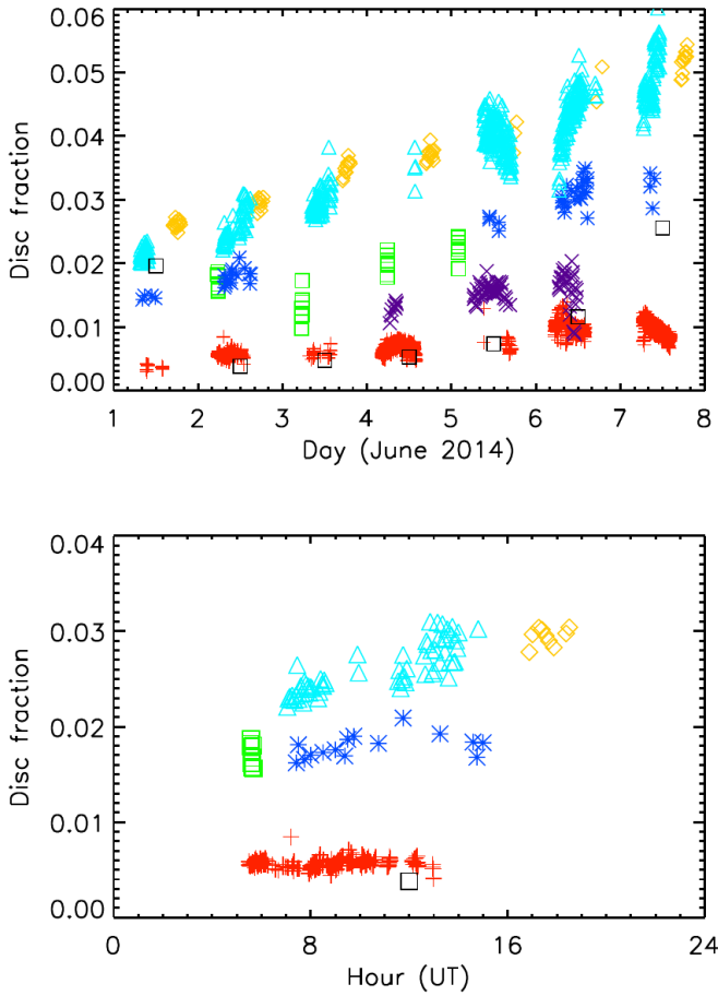
Fig. 10. Plage areas in disc fraction as a function of time from the datasets of Ba (green squares), Br (blue asterisks), CL (purple x symbols, only in the top panel), Ka (red plus signs), ML (orange rhombuses), and Te (cyan triangles). Shown are results for individual images over the course of the first week in June 2014 (top panel) and over the course of 02 June 2014 (bottom panel). Also shown are the sunspot areas by Balmaceda et al. (2009, black squares) multiplied by 10 to bring them to roughly the same level as the plage areas for the sake of comparison.
