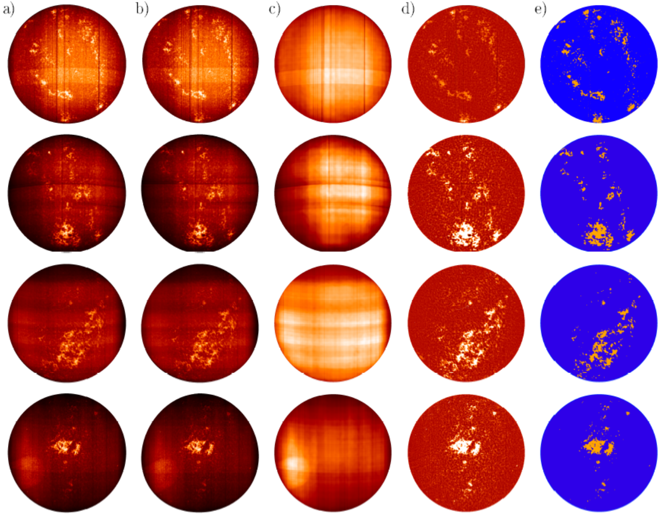
Fig. A.1. Examples of processing steps applied on Ky observations taken on 22/10/1937 (1st row), 28/10/1939 (2nd row), 21/01/1959 (3rd row), and 30/04/1961 (4th row). Columns are: original raw density image (a), density image resampled to straighten the arcs (b), computed background of the original image (c), photometrically calibrated and limb-darkening-compensated image (d), and segmentation mask (e). The raw density images and the backgrounds are shown to the entire range of values within the disc, the calibrated images are shown in the range [-0.5, 0.5] , while the masks show plage regions in orange and QS and network regions in blue. The images are not compensated for ephemeris.
