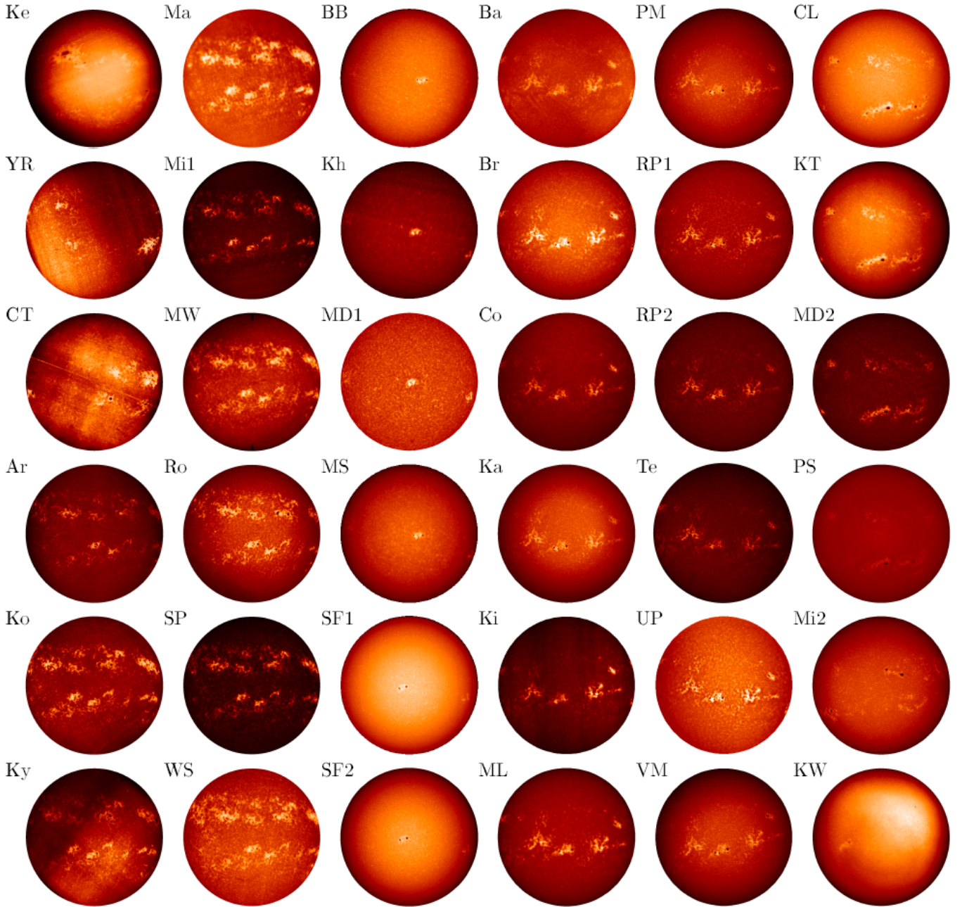
Fig. 1. Examples of observations from the various archives analysed in this study, except from MM and Sc. With the exception of the images in the first and last column, the images within each column correspond to roughly the same day. Within a column the images are shown in alphabetical order according to the name of the observatory, given by a 2-letter abbreviation, with a numeral added in some cases (see Table 1 for the corresponding observatory name). In particular, the dates of the observations are: 14/07/1892 for Ke; 16/02/1907 for YR; 04/09/1908 for CT; 03/02/1968 for Ma; 04/02/1968 for Ko, Ky, Mi1, MW, and SP; 05/02/1968 for Ar, Ro, and WS; 16/07/1995 for BB, Kh, MD1, and MS; 15/07/1995 for SF1 and SF2; 13/03/2014 for Ba, Br, Co, Ka, Ki, ML, PM, RP1, RP2, Te, UP, and VM; 01/08/2012 for CL, KT, MD2, and PS; 10/07/2015 for Mi2; 23/04/2018 for KW; respectively. The images are shown after the preprocessing to identify the disc and re-sample them to account for the disc's ellipticity (when applicable) and convert the historical data to density values. The images have been roughly aligned to show the solar north pole at the top.
