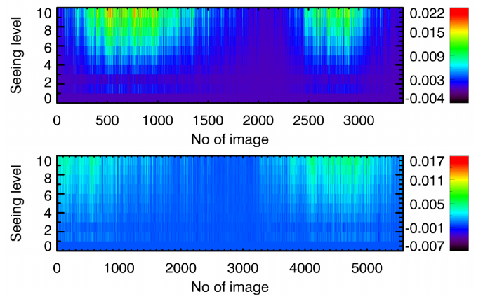
Fig. 11. Colour-coded difference in fractional plage areas derived from RP1 (top) and MD1 (bottom) images downgraded to simulate effects of seeing and those derived from the original RP1 and MD1 images, respectively. The MD1 data used here are only those taken with a CCD camera between 2002 and 2017. Each row (column) of boxes shows results derived from a given observation (width of the smoothing Gaussian function). See Section 4 for details.
