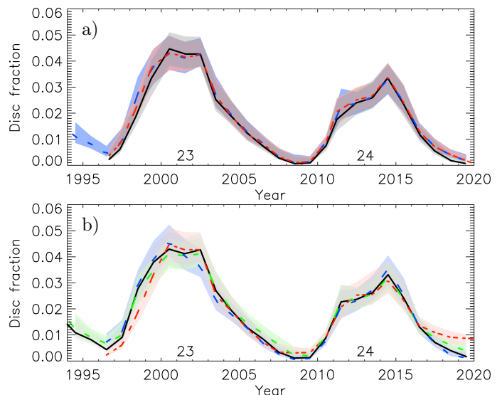
Fig. 15. Top: RP1 plage area series (solid black) plotted along with the RP1 backbone composite series used in our plage area composite (dashed blue) and RP1 backbone composite series keeping only the days common with the RP1 individual series (dashed red). Bottom: RP1 backbone composite series when varying the included individual datasets based on their bandwidth. The different curves show the RP1 backbone composite by keeping Ba, Co, Kh, RP2, SF1, SF2, Te, Up (dashed green), Br, ML, BB (dashed blue) and Ka, PM, VM (dashed red). The RP1 backbone series used for our composite is shown in solid black. Depicted are annual median values (solid lines) along with the 1\sigma asymmetric intervals (shaded surfaces). The SC numbers are given below the curves.
