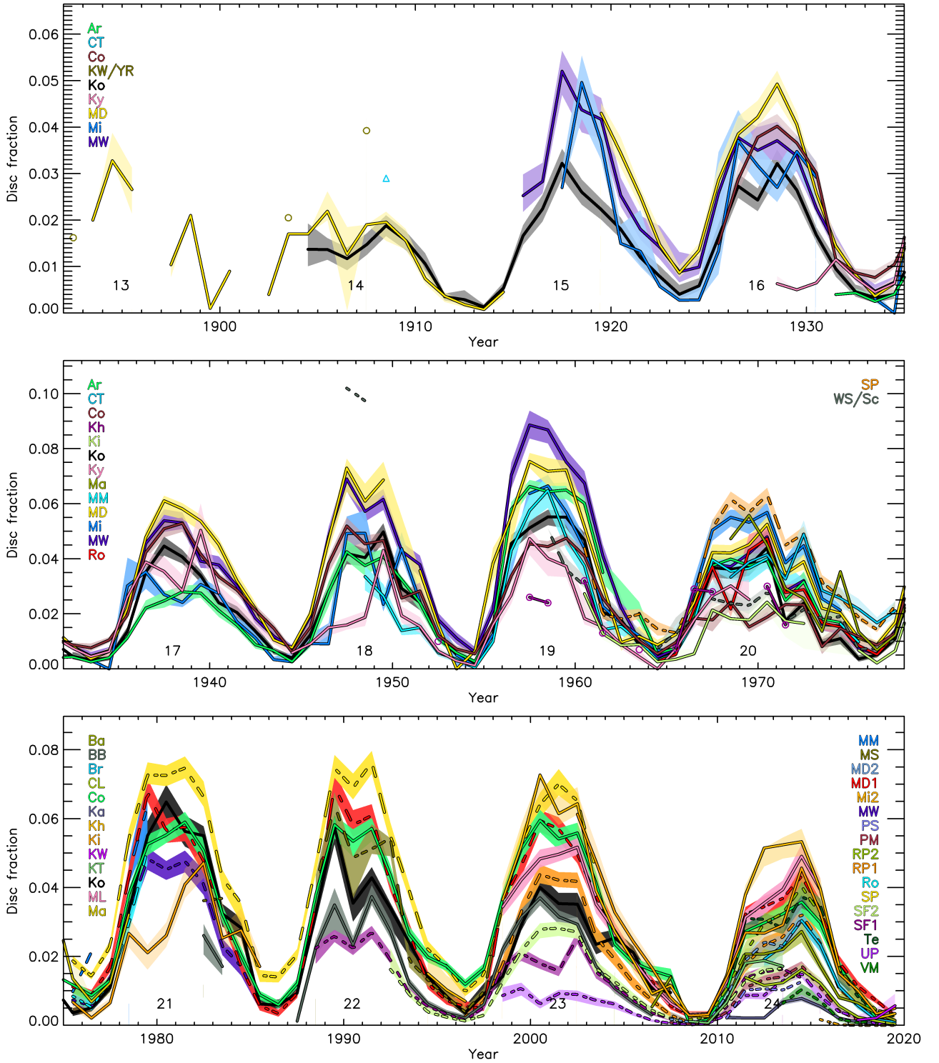
Fig. 7. Evolution of plage areas given as fraction of the solar disc derived from analysis of the 38 datasets considered in this study. Shown are annual median values (lines) along with the asymmetric 1\sigma interval (shaded surfaces) for each dataset as specified in the legend. To improve visibility, the archives listed in the legend in the right side of the plot are represented by dashed lines. Due to the scarcity of observations, the plage areas derived from the Ke/YR and CT observations in the top panel, as well as the Kh in the middle panel are represented by circles, triangles, and circles, respectively. The conventional solar cycle (SC) numbers are given below the curves.
