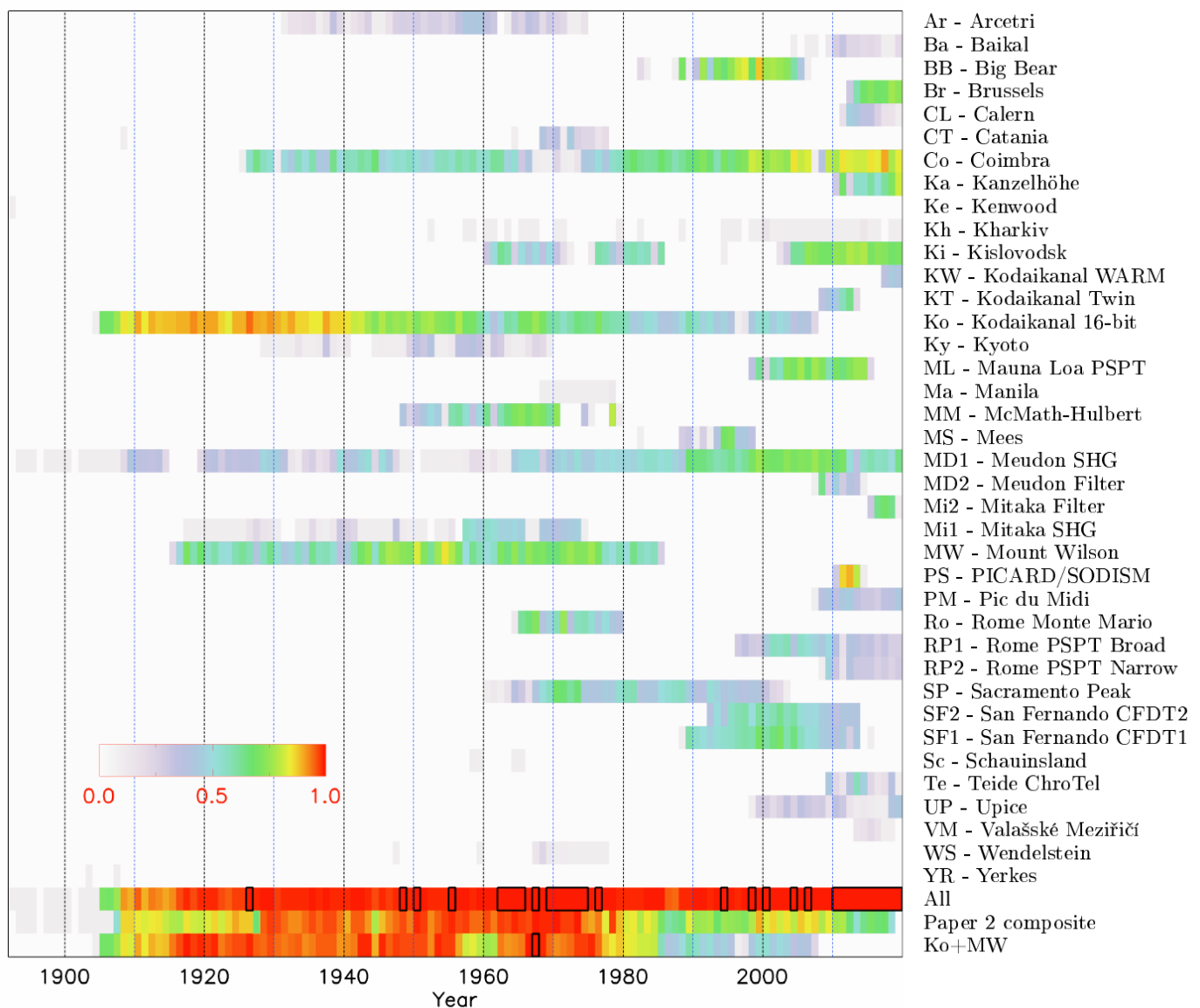
Fig. 2. Annual coverage of the various Ca II K archives analysed in this study, except from those taken off-band (see Sect. 2 for details). Also shown is the annual coverage of all the archives combined, the one for the Chatzistergos et al. (2019b, paper 2) composite series, and the annual coverage when only Ko and MW are considered. The annual coverage is colour-coded as shown by the colour bar plotted in the bottom left corner of the panel. Years with full coverage are outlined with black rectangles.
