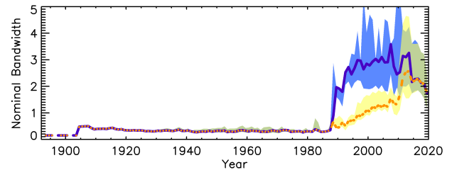
Fig. 3. Average nominal bandwidth from all 38 archives included in this study (solid purple) as well as from all archives excluding SF1 and SF2 (dashed orange). The shaded areas show the 1\sigma uncertainty.
