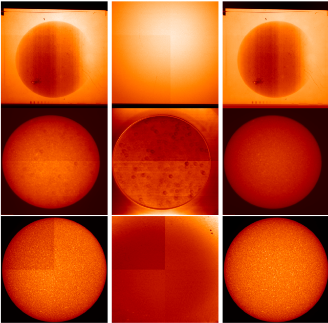
Fig. 4. Examples of raw images (left column), data employed for the calibration of the CCD recording device (middle column), and calibrated images (right panels) from the Ko (first row), MS (middle row), and RP1 (bottom row) archives taken on 19/08/2006, 19/12/1995, and 28/02/2020, respectively. The images have not been compensated for ephemeris and are shown in their entire range of values.
