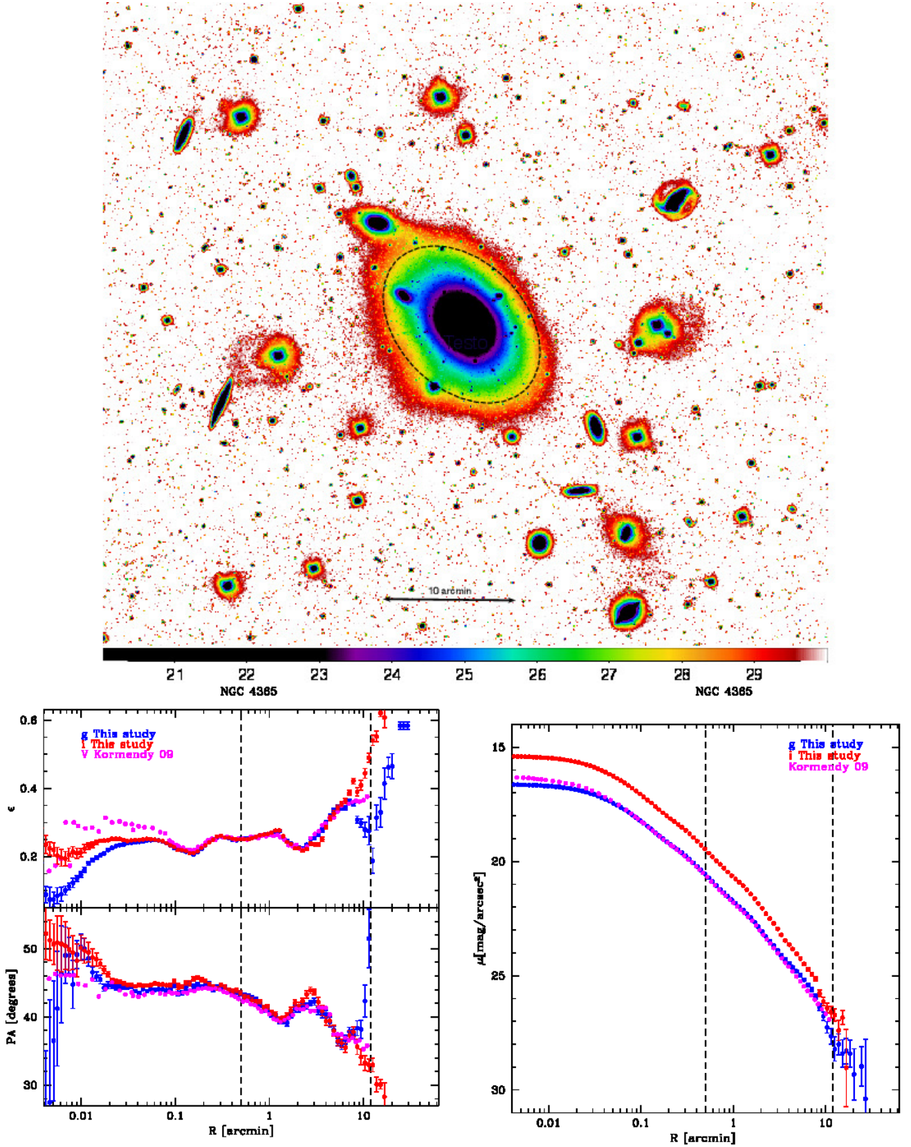
Fig. D.2. Same as Fig. D.1 for NGC 4365. The V-band surface brightness profile by Kormendy et al. (2009, magenta points in the bottom panel) was shifted by +0.2 mag to match the amplitude of the VEGAS profile.
