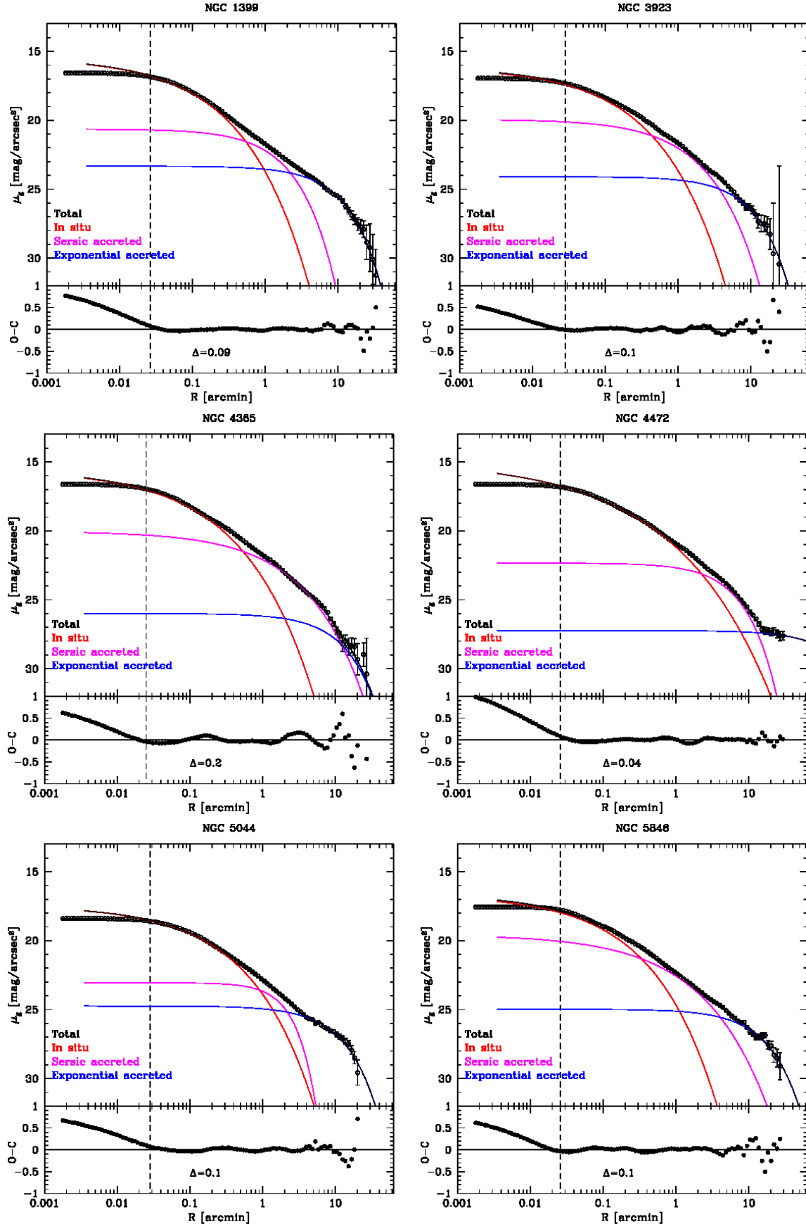
Fig. D.9. VST g-band profiles of NGC 1399, NGC 3923, NGC 4365, NGC 4472, NGC 5044, and NGC 5846, fitted with a three-component model motivated by the predictions of theoretical simulations.
