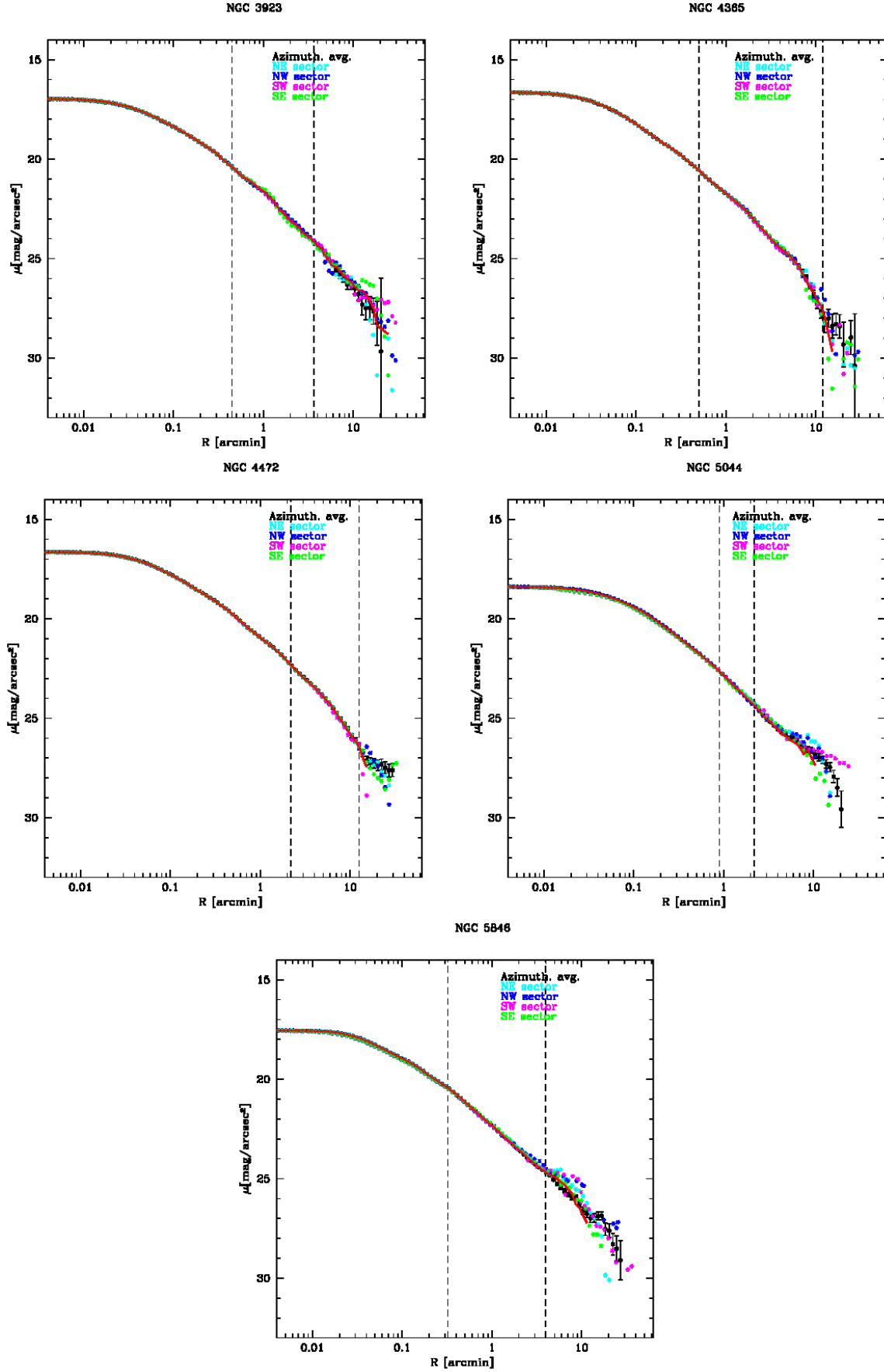
Fig. B.1. VST g-band surface brightness profiles of NGC 3923, NGC 4365, NGC 4472, NGC 5044, and NGC 5846, extracted in azimuthal sectors and compared with the azimuthally averaged profile. The red line is the average profile, while the dashed lines indicate the location of the transition radii.
