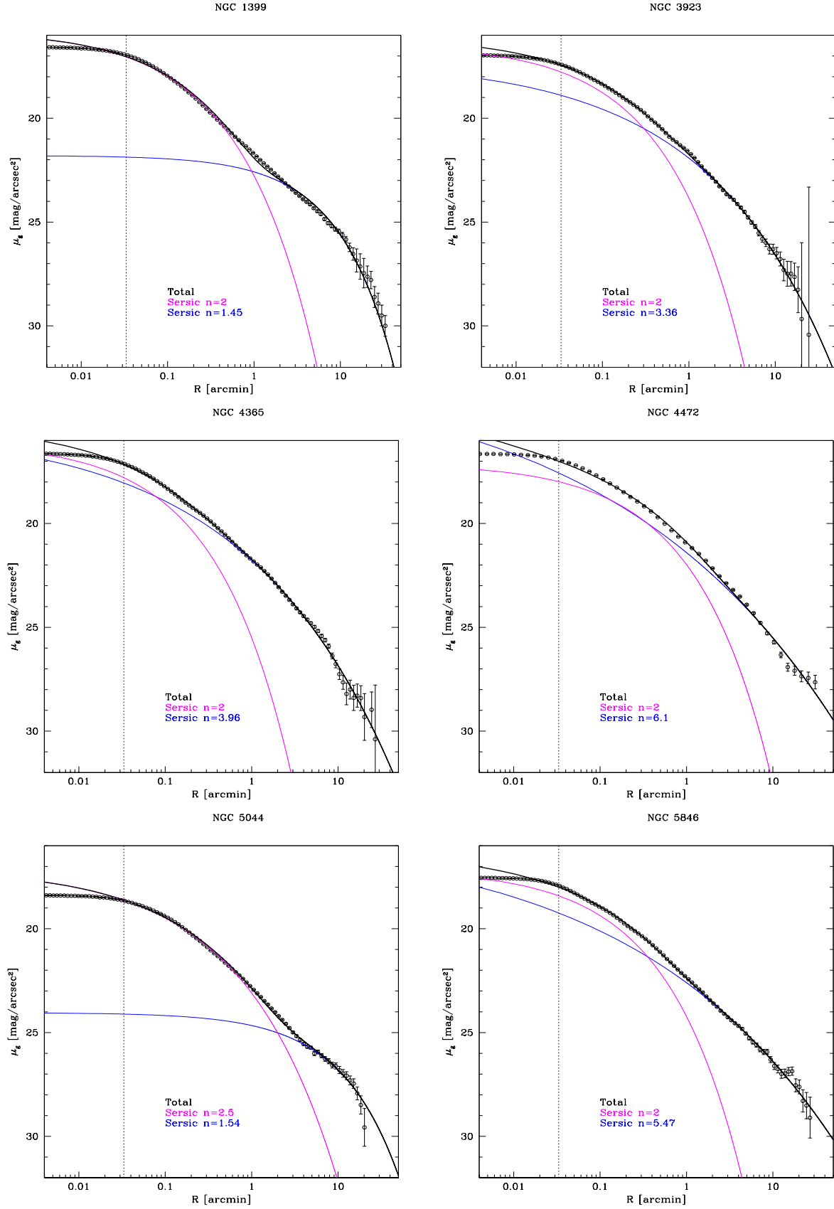
Fig. C.1. VST g-band profiles of NGC 1399, NGC 3923, NGC 4365, NGC 4472, NGC 5044, and NGC 5846 plotted on a logarithmic scale. The blue line indicates a fit to the outer regions. The magenta line indicates a fit to the inner regions with a Sérsic profile with n fixed from theory (Cooper et al. 2013), and the black line indicates the sum of the components in each fit. The dotted line indicates the core of the galaxy ( R \sim 2 arcsec), which was excluded in the fit.
