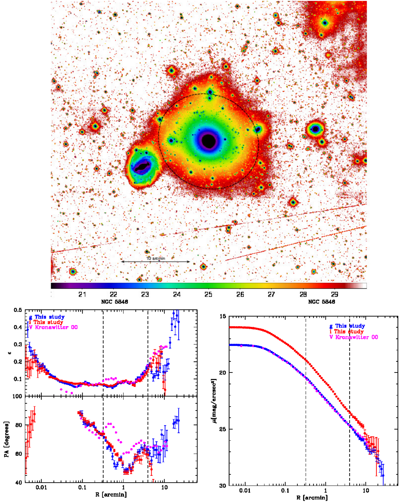
Fig. D.5. Same as Fig. D.1 for NGC 5846. The V-band surface brightness profile by Kronawitter et al. (2000, magenta points in the bottom panel) was shifted by +0.23 mag to match the VEGAS result.
