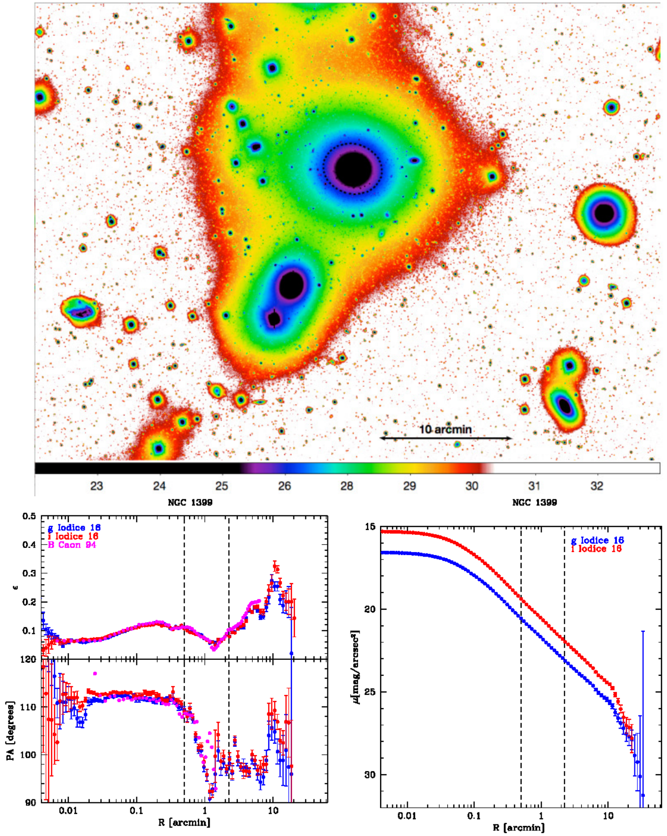
Fig. 1. Top: VST g-band sky-subtracted image of the field around NGC 1399. The colour scale represents surface brightness in \text{mag}/\text{arcsec}^2 . The dashed black contour indicates the transition radius in the surface brightness profile, defined in Sect. 5. North is up, east is to the left. Bottom left: ellipticity ( \epsilon ) and position angle (PA) profiles for NGC 1399, in the g band (blue points) and i band (red points). Bottom right: azimuthally averaged surface brightness profiles in the g (blue) and i (red) bands. The dashed lines indicate the transition radii in the surface brightness profile, listed in Table 6, which represents the location of the transition between two fit components, as described in Sect. 5.
