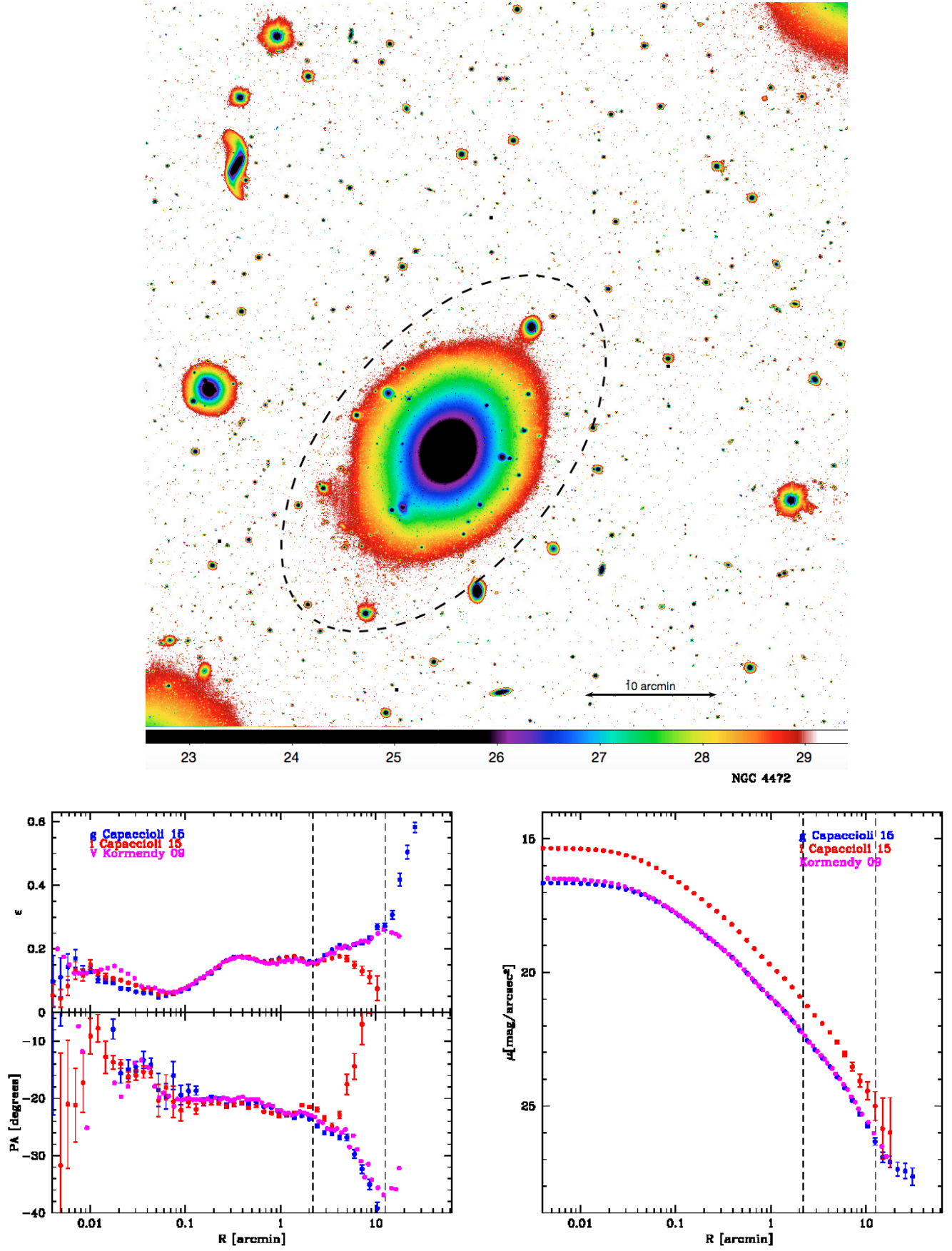
Fig. D.3. Same as Fig. D.1 for NGC 4472. The V-band surface brightness profile by Kormendy et al. (2009, magenta points in the bottom panel) was shifted by +0.33 mag to match the amplitude of the VEGAS profile.
