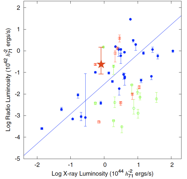
Figure 6. The total radio luminosity from radio-jets vs X-ray luminosity of the ICM (without any AGN X-ray contribution) plot from Mittal et al. (2009) for strong cool-core ( t_{\text{cool}} < 1 \text{ Gyr} ; filled blue circles), weak cool-core ( 1 \text{ Gyr} < t_{\text{cool}} < 7.7 \text{ Gyr} ; open green circles) and non cool-core ( t_{\text{cool}} > 7 \text{ Gyr} ; open red squares) clusters, with t_{\text{cool}} representing their central cooling times. CL J1449+0856 has been represented here with the red ‘★’. The observational error bars denote the systematic variation introduced with the change of the \alpha used in the calculation of the radio luminosity. We use 0.7 (the average for star formation) as the lower limit, while for the upper limit we have 1.5 (limit estimated using the 325 MHz GMRT observation).
