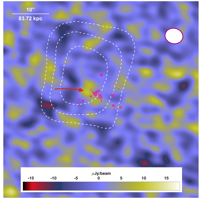
Figure 7. ALMA 92 GHz residual image of CL J1449+0856 borrowed from Gobat et al. (2019) , after subtracting both the point sources and the SZ signal from the cluster (denoted by the white dashed contours). The colour bar at the bottom denotes the residual flux per beam with a positive signal indicating a lack of gas density and vice-versa. This has been overlaid with the radio contours in magenta while the white-filled red ellipse shows the size of the synthesised ALMA beam. The red arrow points to the possible under-density due to the jets.
