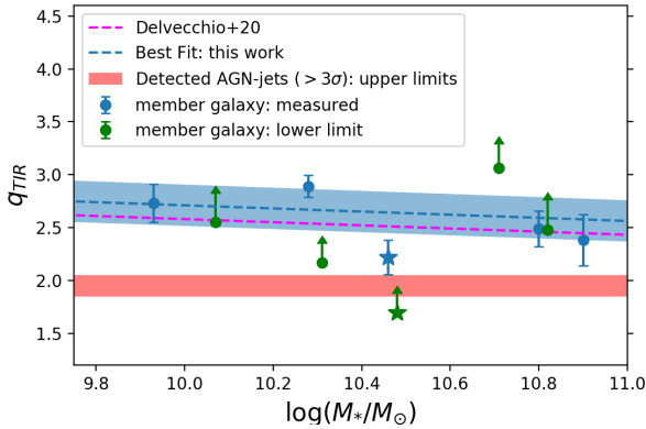
Figure 4. The total infrared and radio luminosity ratio ( q_{\text{TIR}} ) vs the stellar mass of the member galaxies of CL J1449+0856 (listed in Table. 1), with the two AGNs shown with the ‘★’ marker. We also plot the best fit along with the 1\sigma limits. We only provide the lower limit q_{\text{TIR}} for the galaxies lacking a radio detection which are obtained using the 2\sigma upper limits of the 3 GHz VLA data. The slope was fixed to the value determined in Delvecchio et al. (2020), the q_{\text{TIR}} vs. M_* relation from which has also been presented for comparison. Finally, the q_{\text{TIR}} upper limits of the AGN radio-jets detected ( > 3\sigma ) in this work has also been shown.
