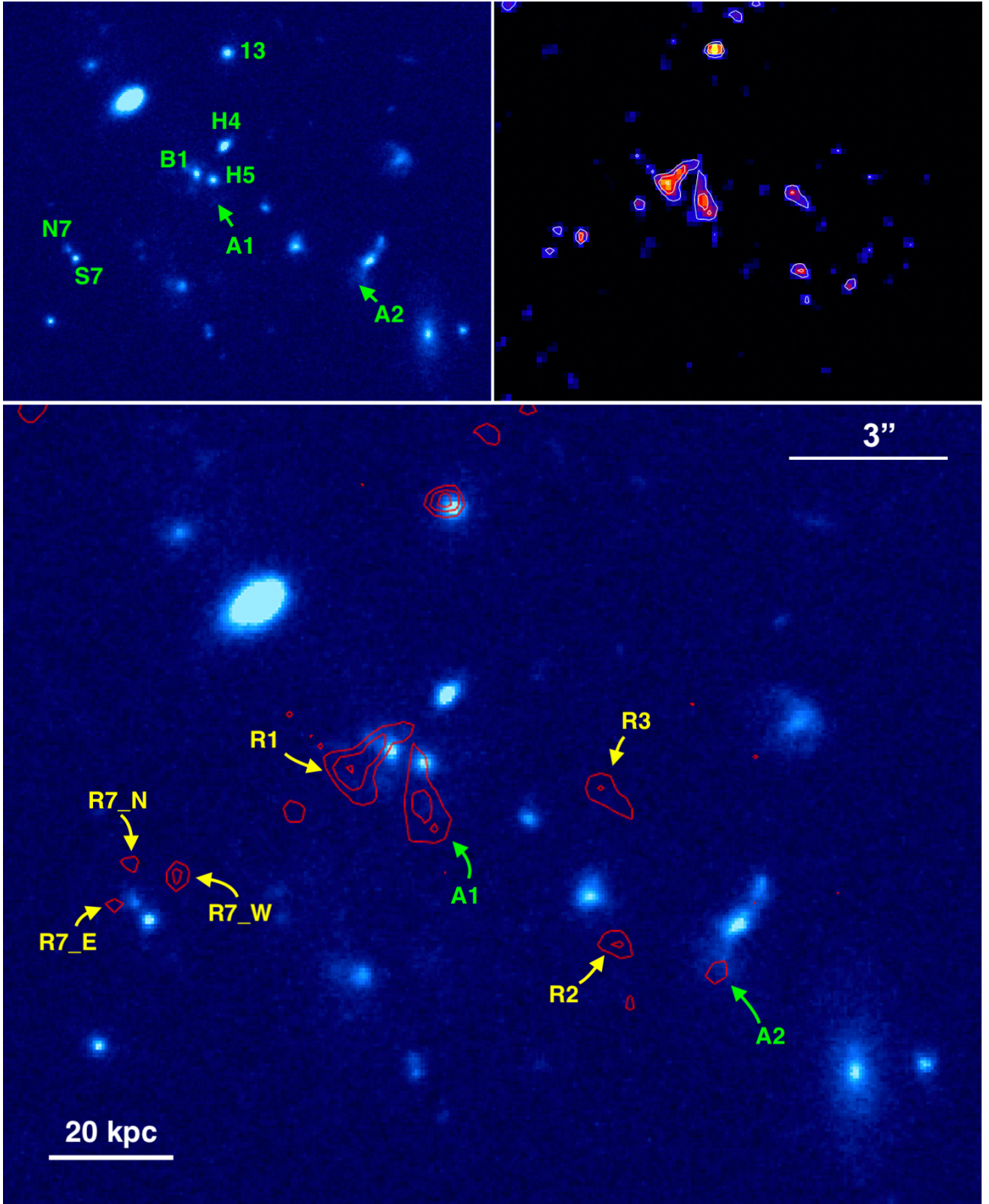
Figure 5. (Top-left) The HST /WFC3 F140W image with the sources listed in Table 1 marked. However, 2 and A6 are not shown as they are outside the area shown and are not relevant to the results presented in this work. (Top-right) The 3 GHz VLA image of the region with sigma contours starting at 3\sigma with 1\sigma increments, as in Fig. 3. (Bottom) The same HST /WFC3 F140W image with the contours of the VLA 3 GHz image along with the AGN-jets listed in Table 2 (in yellow) and the two HST undetected bright ALMA sources A1 and A2 that are also detected at 3 GHz (in green) marked.
