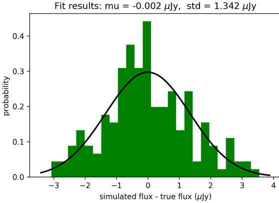
Figure 2. The histogram created out of the source detection simulation carried out within a distance of \sim 80'' from the centre of CL J1449+0856 on the VLA 3 GHz image. The x-axis gives the difference between the measured flux of the simulated sources and their true values, while the y-axis provides a measure of the fractional occurrence. We fit a gaussian, the \sigma of which is the RMS noise/beam of in the data
