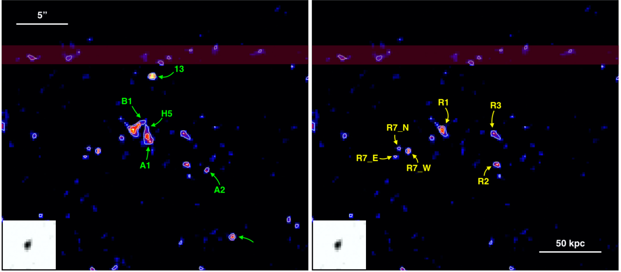
Figure 3. (Left) The VLA 3 GHz image of the cluster core with the galaxies in Table 1 detected ( > 3\sigma ) with an additional bright interloper and (right) the subsequent residual image after their subtraction, with the remaining major emission regions marked. The sigma contours in white are also provided for each of the images, starting from 3\sigma with increments of 1\sigma . Finally, the white boxes show the VLA 3 GHz PSF in the same spatial scale as that in the images. The maroon shaded region highlights a very faint imaging residual spike from the strongest source in the VLA field of view, which contributes to a few spurious \sim 3\sigma peaks. No such systematics are present in the rest of the image.
