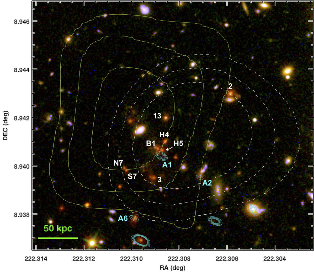
Figure 1. HST /WFC3 color composite image of CL J1449+0856. The grey dashed contours represent the X-ray intensity map from Chandra (Valentino et al. 2016) while the extended green contours display the SZ signal tracing the mass distribution (Gobat et al. 2019). The cyan contours are the 870\mu\text{m} ALMA sources. All galaxies listed in Table 1 have been marked.
