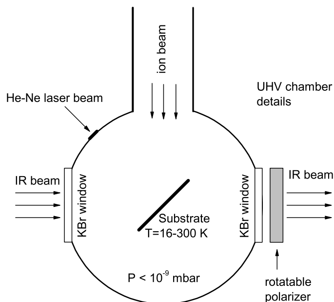
Fig. 1. Schematic depiction of the UHV chamber.
