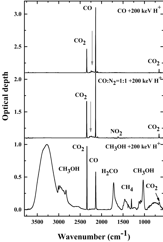
Fig. 2. Selected infrared spectra, in the range 3800–560 cm -1 , used in the fitting procedure. From top to bottom the spectra refer to pure CO after bombardment with 200 keV H + at 16 K, a mixture CO:N 2 = 1:1 after bombardment with 200 keV H + at 16 K, and pure CH 3 OH after bombardment with 200 keV H + at 16 K. Spectra are normalized to their maximum optical depth value and are shifted for clarity. The main features formed after bombardment are labelled. The vertical grey arrows indicate the spectral range where most of the features assigned to carbon chain oxides and nitrogen oxides occur. A detailed description of these spectra is given by Palumbo et al. (2008), Sicilia et al. (2012), and Modica & Palumbo (2010).
