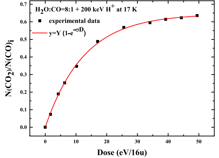
Fig. 3. Column density of CO 2 divided by the initial column density of CO after ion bombardment with 200 keV H + of a H 2 O:CO = 8:1 mixture at 17 K. Experimental data are fitted by an exponential curve.
