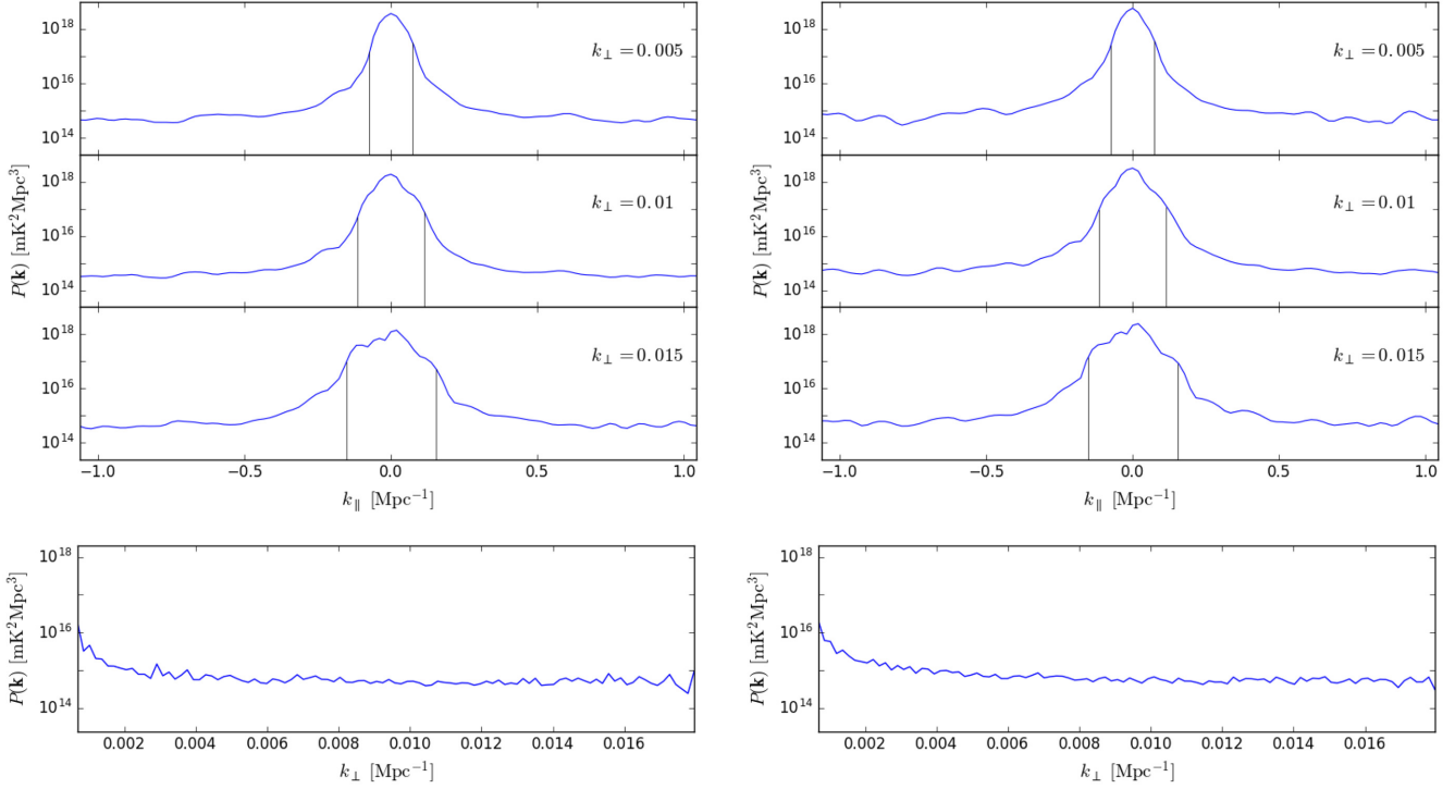
Figure 4. Vertical and horizontal cuts through the power spectra in the top row of Fig. 3. The top row panels contain three vertical cuts made at k_{\perp} values of 0.005, 0.01, and 0.015 \text{Mpc}^{-1} . The black lines indicate the location of the horizon at these k_{\perp} values. The bottom row shows a horizontal cut made at k_{\parallel} = 0.53 \text{ Mpc}^{-1} . The left column is from power spectra generated from polarization XX and the right column from polarization YY.
