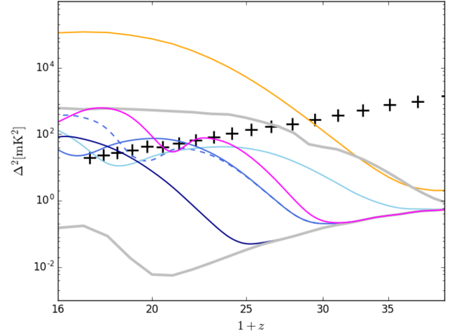
Figure 10. The simulated noise level of OVRO-LWA from 3000 h of partially coherently integrated observations at k = 0.3 \text{ Mpc}^{-1} (crosses), plotted on top of a selection of 21-cm models (note the x-axis is in log scale). We show standard models with V_c = 4.2 \text{ km/s} (light blue), 24.2 \text{ km/s} (blue), and 52.1 \text{ km/s} (dark blue) for fixed values of f_* = 3 per cent, f_X = 0.07 , \alpha = 1.5 , and \nu_{\min} = 0.1 \text{ keV} (the EoR parameters, although they do not matter much at these redshifts, are chosen to be R_{\text{mfp}} = 30 \text{ Mpc} and \tau = 0.064 ). For comparison, we also show the case of higher f_X = 1.7 for V_c = 24.2 \text{ km/s} (dashed blue). We also show the model with maximum signal to noise in the LEDA band (magenta, out of examined 11164 models). This case has the following values of the astrophysical parameters: f_* = 50 per cent, V_c = 35.5 \text{ km/s} , f_X = 1 with \alpha = 1.5 and \nu_{\min} = 0.1 \text{ keV} , R_{\text{mfp}} = 40 \text{ Mpc} , and \tau = 0.07 . We also show the envelope of all possible signals in the standard astrophysical scenario (thick grey lines, Cohen, Fialkov & Barkana 2018). Finally, we show an external radio background model (orange) that has the maximum signal to noise for LEDA: f_* = 12 per cent, V_c = 4.2 \text{ km/s} , f_X = 0.01 with hard X-ray SED, \tau = 0.056 , and the excess radio background of 1.2 per cent over the CMB at 1.42 GHz (from Fialkov & Barkana 2019).
