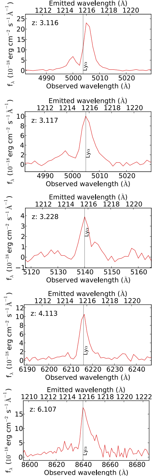
Fig. 9. Full-resolution MUSE 1D spectrum of sources (top to bottom) 49, 50, 51, 52, and 53, with wavelength on the horizontal axis and the flux on the vertical axis. The spectra are zoomed in on the Ly \alpha line, which is indicated by the vertical black line. For source 49, we determined the redshift based on other UV-emission lines, while for the other sources we used Ly \alpha to determine z . For sources 49, 52, and 53 the different images of the same source are stacked to optimise the signal-to-noise ratio. The fluctuations and non-zero continuum around Ly \alpha in object 53 are the result of locally increased noise.
