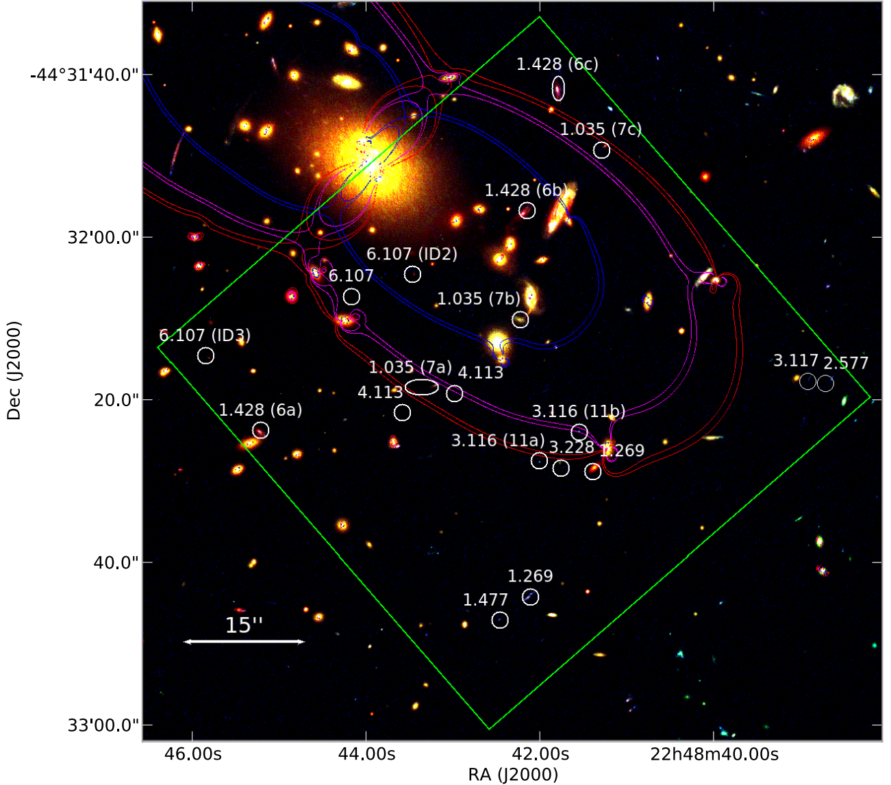
Fig. 1. Red-green-blue image composition of HST images of the part of AS1063 that we observed with MUSE, where the colours in this image are blue = F435W + F475W , green = F606W + F625W + F775W + F814W + F850LP , red = F105W + F110W + F140W + F160W . The individual HST images were obtained and distributed by the CLASH collaboration. The green square delimits the 1 \times 1' MUSE FOV. All 19 objects with a spectroscopic redshift z > 1 are shown as white circles and their redshifts. Numbered galaxies were noted before by Monna et al. (2014) and Balestra et al. (2013). The blue, magenta, and red contours correspond to regions where the magnification is \mu > 200 at z = 1, 2 , and 4 , respectively. The magnifications are based on the second version of the Sharon models (Johnson et al. 2014), which were chosen for illustrative purposes, but we note that this is only one out of many different available models.
