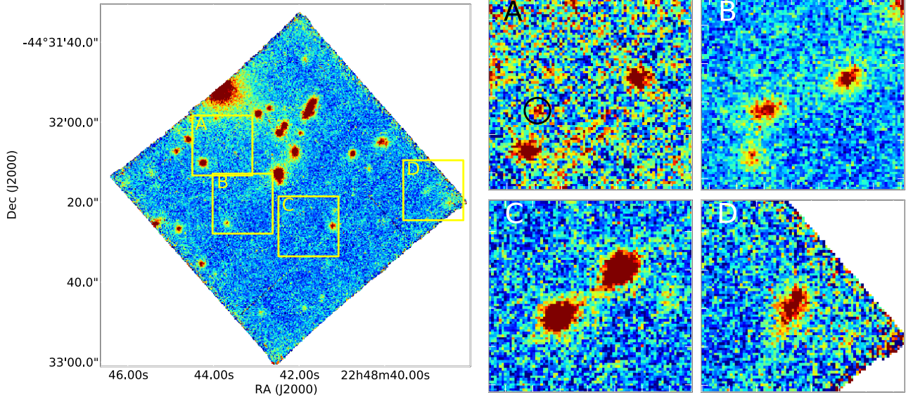
Fig. 2. Snapshot of our MUSE pointing towards Abell S1063. Left: a slice of reduced MUSE data cube centred at 7250 \text{ \AA} with \Delta\lambda = 1.25 \text{ \AA} . Right: zoom-ins of the four regions with LAEs marked on the left panel, where the wavelength is centred at the peak of \text{Ly}\alpha for galaxies 53a,c 52a,b, 49a,b, and 50 in panels A, B, C, and D, respectively. In zoom-in A, we placed a circle around the weak additional detection of the quintuply lensed galaxy at z = 6.107 .
