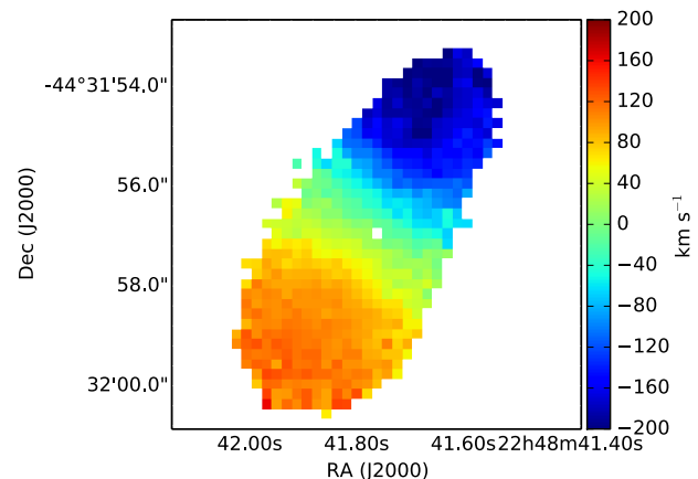
Fig. 7. [O II] velocity map of galaxy 38 at z = 0.607 . The coordinates are shown on the axes, and the velocity is for every pixel by its colour. This figure clearly illustrates the power of MUSE for 2D spectroscopy.
