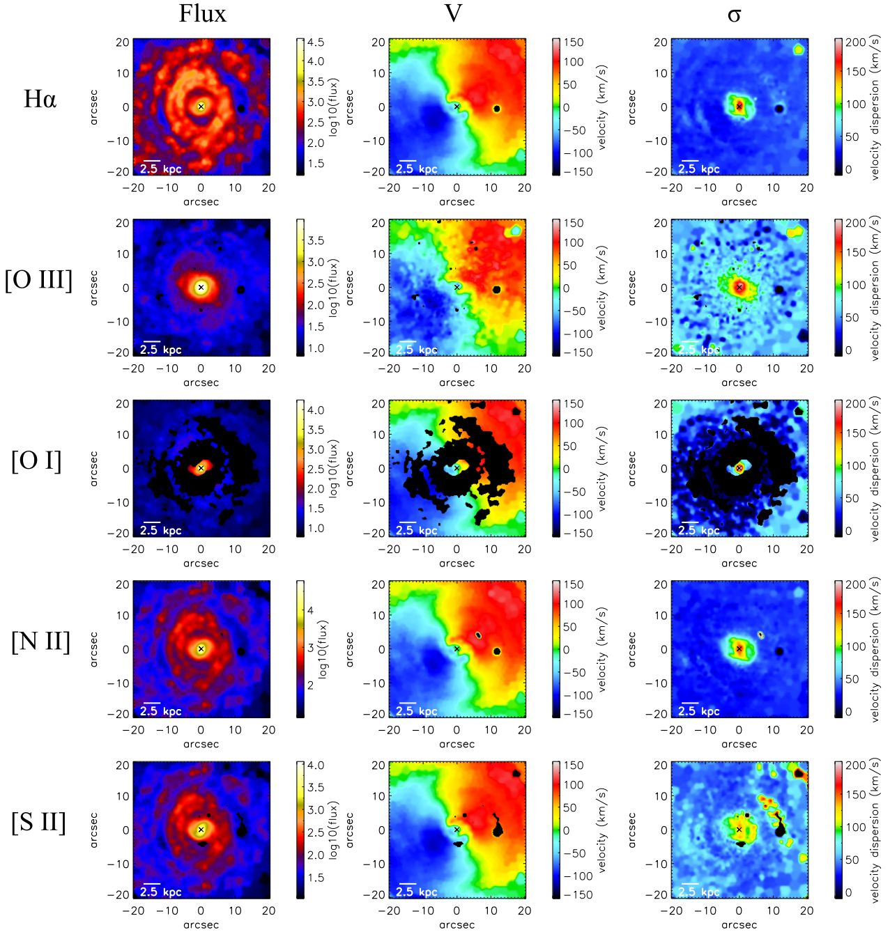
Figure 8. Maps of ionized gas tracers. Each row corresponds to a different tracer, from top to bottom: \text{H}\alpha , [O III], [O I], [N II], and [S II]. Only the narrow components of the lines are shown in the panels. Columns from left to right show the line flux (in a logarithmic scale for visualization purposes), velocity and velocity dispersion maps, respectively. The black cross indicates the AGN position as determined from the \text{H}\alpha broad emission line peak flux. North is up, East is left. The regions in black have been masked out due to low S/N (see the text for details).
