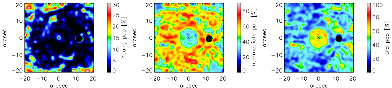
Figure 17. Fraction of stars in three stellar age bins. Left: Young age stars (<1 Gyr). Centre: Intermediate age stars (1 Gyr < age < 5 Gyr). Right: Old age stars (> 5 Gyr).
