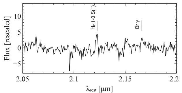
Figure 2. Nuclear K -band spectrum obtained from the mean of the spectra within the central 0.5 \times 0.5 \text{ arcsec}^2 . The spectrum has been spectrally binned by a factor of 2 and rescaled for visualization purposes by subtracting the mean flux value. The H_2 1-0 S(1) 2.12 \mu\text{m} emission that traces warm molecular gas is observed in the spectrum.
