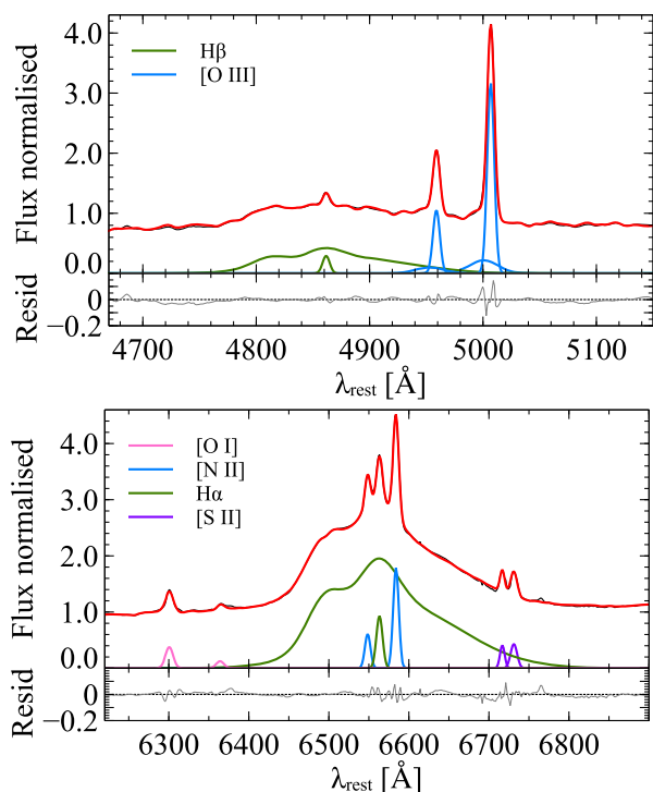
Figure 1. Example of the emission line fitting procedure in the nucleus of Mrk 590. The nuclear spectrum was extracted from a nuclear region of size 0.8 \times 0.8 \text{ arcsec}^2 . The top panel shows the GANDALF fit for the H\beta spectral region while the bottom panel shows the H\alpha spectral region. In each panel the galaxy spectrum is shown at the top and the residuals at the bottom. The galaxy spectrum is shown in black with the best-fitting model shown in red. The flux has been normalized. The individual line components are illustrated by the coloured lines. In the top panel the green lines show the broad and narrow H\beta emission line components while the blue lines show the broad and narrow [O \text{ III}] emission line components. In the bottom panel the broad and narrow H\alpha emission line components are shown in green and the [O \text{ I}] , [N \text{ II}] , and [S \text{ II}] emission lines in pink, blue, and purple, respectively.
