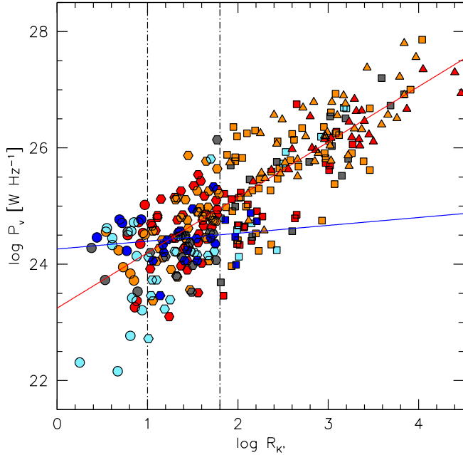
Fig. 11. Behavior of radio power P_v in units of W as function of Kellermann's parameter R'_K . Symbol coding corresponds to different radio morphologies and to different STs. Triangles: RL FRII; squares: RL CD, exagons: CD RI, circles: CD RQ. Red: union of B1^{+++} and B1^+ , orange: B1, gray: A1, pale blue: A2, xA: blue. The lines trace unweighted least square fits for Pop. B sources (red) and for xA sources considered over the three radio loudness classes.
