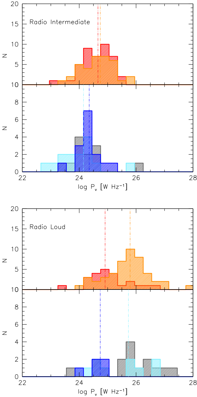
Fig. 10. Distribution of radio power P_v in units of W for RI (top) and RL (bottom), for different spectral types along MS. Top panels: distributions for the union of B1 ++ and B1 + (red), B1 (orange) spectral types, the bottom ones for A1 (gray), pale blue (A2), and xA (blue). The vertical dot-dashed lines mark the medians of the Pop. B (red and orange), A2 (pale blue) and xA (blue) distributions.
