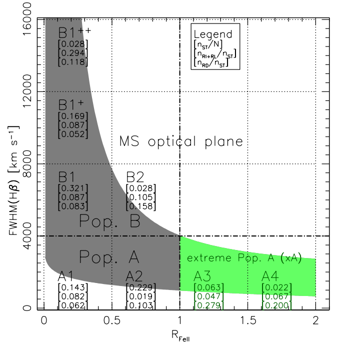
Fig. 1. Sketch illustrating definition of STs along MS, as function of R_{\text{FeII}} and FWHM(H \beta ). The numbers in square brackets yield from top to bottom, the prevalences of each spectral bin ( n_{\text{ST}} ) in an optically selected sample (Marziani et al. 2013), of the RI and RL sources ( n_{\text{RI+RL}} ) and of RD ( n_{\text{RD}} ) in each spectral bin. The total number of sources is N = 680 . The gray and pale green areas trace the source occupation in the plane; the green area separates extreme Population A from the rest of the MS.
