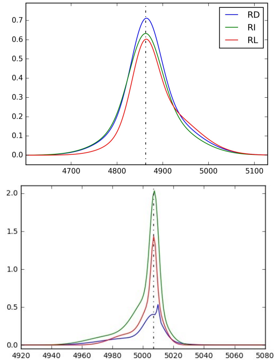
Fig. 8. CD B1 H \beta (top) and CD A2 [OIII] profiles (bottom) for different radio power classes. Blue refers to the RD class, green to the RI one and red to the RL one.
