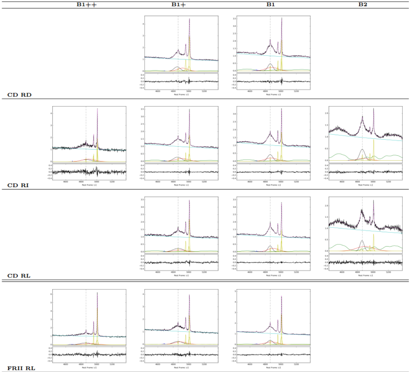
Fig. 3. Composite of STs along MS, ordered from B1^{++} to B2 . Each panel shows the original composite, along with the modeled continuum (cyan line). The lower part of the panels shows the result of the specfit analysis on the emission lines. H\beta_{BC} : black line, H\beta_{VBC} : red line; FeII: green line; yellow lines: H\beta narrow components and [OIII]\lambda\lambda 4959, 5007 .
