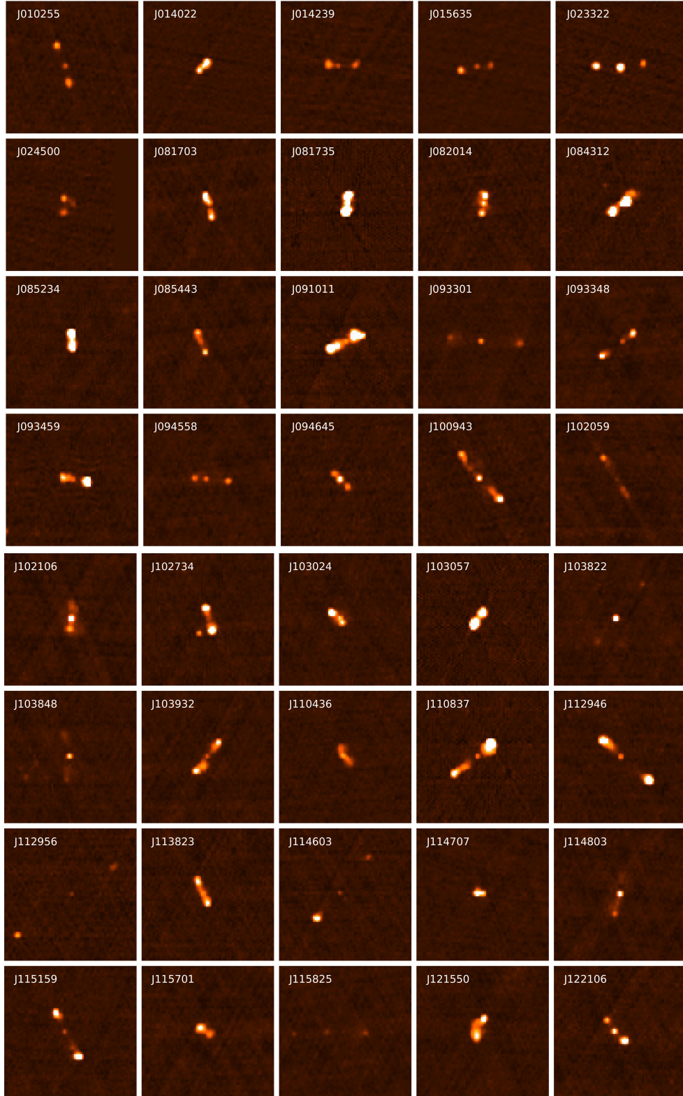
Fig. A.1. Radio maps at 1.4 GHz for FRII sample from FIRST catalog with size of field 4.5' \times 4.5' and Maximum Intensity for Scaling equals to 10 mJy. The images follow the SDSS ID order of Table A.2 from left to right and from top to bottom .
