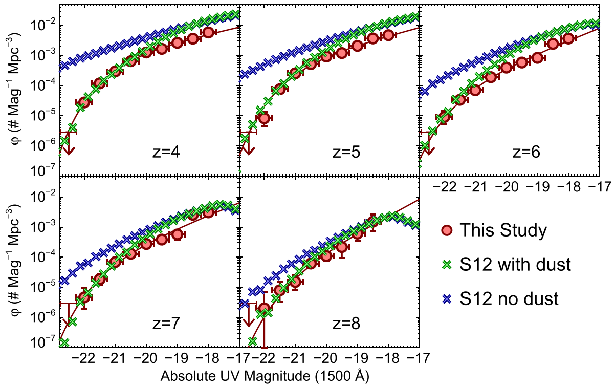
Figure 18. Rest-frame ultraviolet luminosity functions at z = 4 – 8 , comparing our observations to the semi-analytic models (SAMs) of Somerville et al. (2012; S12). The crosses mark the models of S12 both with and without dust. In order for the models to be consistent with the observations, it is clear that some dust is needed at all redshifts (except perhaps at z = 8 ), particularly at the bright end. Using a simple model for dust attenuation, our results suggest that the dust-to-metal ratio or dust geometry must change as a function of redshift, which is a continuation of a trend already pointed out in previous studies. The turnover at very faint luminosities in the SAM predictions is due to the resolution limit of the Bolshoi simulation.
