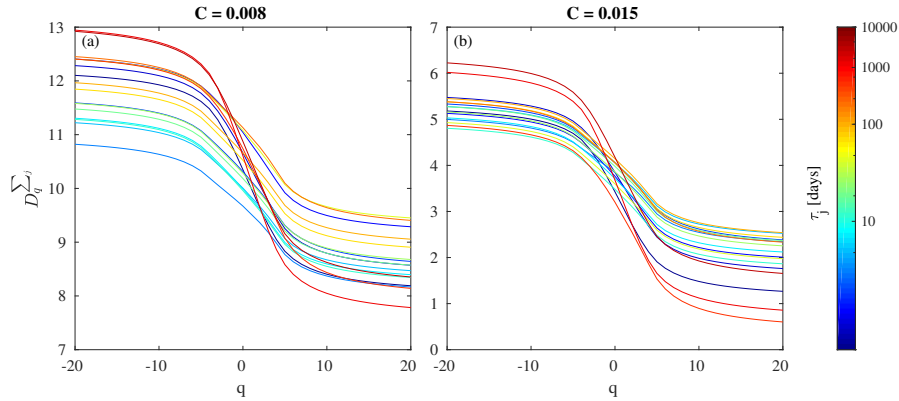
Figure 9. D_{q,\tau} spectra for the coupled ocean-atmosphere dynamics at different timescales \tau_j (indicated by different line colors) for reconstructions of MIMFs summing up from j = 1 to N_j ( D_q^{\sum j} ) for (a) C = 0.008 and (b) C = 0.015 .
