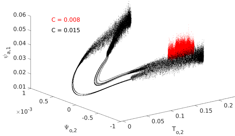
Figure 1. 3-D projection of the full system attractor in the subspace (T_{o,2}, \Psi_{o,2}, \psi_{a,1}) for C = 0.008 (red) and C = 0.015 (black), respectively.
