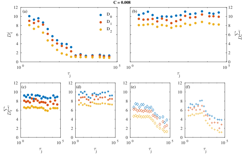
Figure 7. Multiscale capacity dimension D_{0,\tau} , multiscale information dimension D_{1,\tau} , and multiscale correlation dimension D_{2,\tau} for C = 0.008 at different timescales \tau_j for different cases: (a) for each MIMF individually ( D_{0,\tau}^j ), (b) for reconstructions of MIMFs summing up from j = 1 to N_j ( D_{0,\tau}^{\sum_j} ), and (c)-(f) for reconstructions of MIMFs separately for each variable (barotropic modes - (c), baroclinic modes - (d), transport modes - (e), and temperature modes - (f)).
