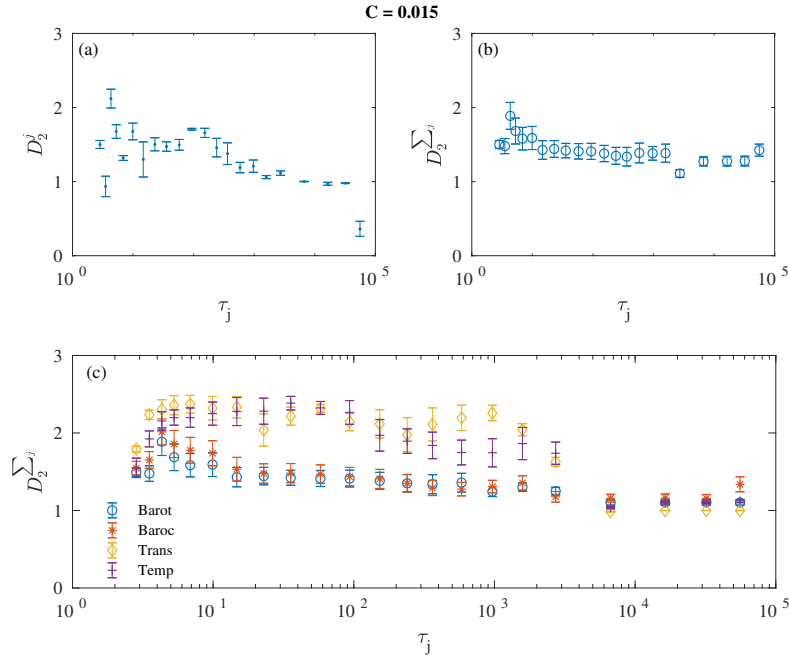
Figure 6. Same as in Fig. 5, but for C = 0.015 .
