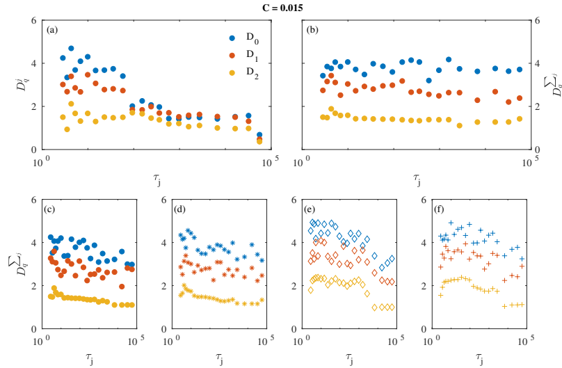
Figure 8. Same as in Fig. 7, but for C = 0.015 .
