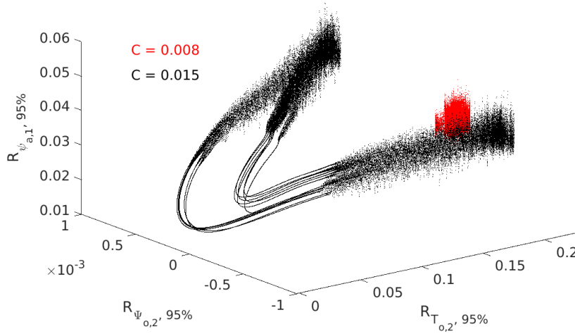
Figure 4. 3-D projection of the full system attractor in the subspace (T_{o,2}, \Psi_{o,2}, \psi_{a,1}) for C = 0.008 (red) and C = 0.015 (black), respectively, as obtained from reconstructions based on the multivariate empirical modes R_{\chi,95\%}(t) accounting for 95% of the total variance of the model dynamics.
