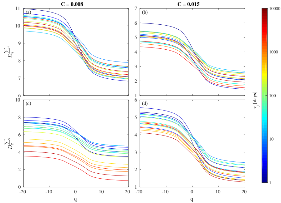
Figure 11. D_{q,\tau} spectra for the dynamics of atmosphere and ocean individually at different timescales \tau_j (indicated by different line colors) for reconstructions of MIMFs summing up from j = 1 to N_j ( D_q^{\sum j} ) for (a,c) C = 0.008 and (b,d) C = 0.015 . Panels (a,b) refer to the atmosphere, (c,d) to the ocean.
