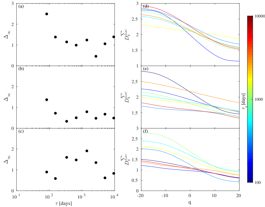
Figure 13. (a)-(c) Multifractal width \Delta_\infty and (d)-(f) D_{q,\tau} spectra at different timescales \tau_j for reconstructions of MIMFs summing up from j = 1 to N_j ( D_q^{\sum_j} ) for (a,d) the North Atlantic, (b,e) the North Pacific, and (c,f) the Tropical Pacific, respectively.
