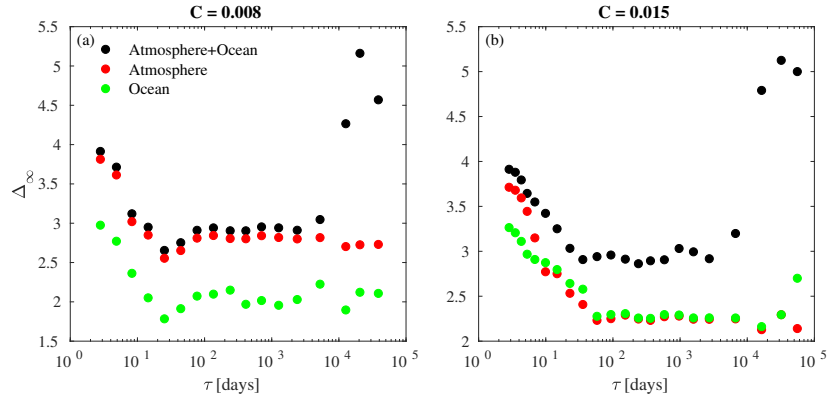
Figure 10. Multifractal width \Delta_\infty at different timescales \tau_j for reconstructions of MIMFs summing up from j = 1 to N_j ( D_q^{\sum j} ) for (a) C = 0.008 and (b) C = 0.015 . The different colors refer to the full system (atmosphere+ocean, black circles), only the atmosphere (red circles), and only the ocean (green circles), respectively.
