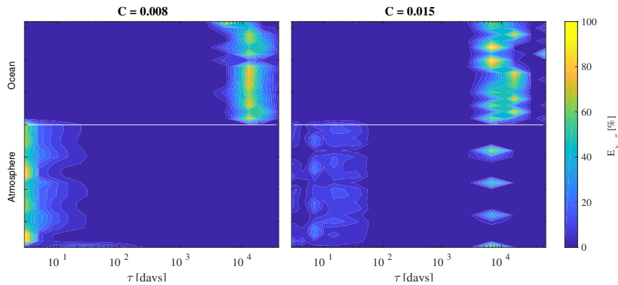
Figure 3. Relative contribution (in percentage) E_{\chi,\tau} of each variable \chi = \{\psi_{a,i}, \theta_{a,i}, \Psi_{o,i}, T_{o,i}\} in dependence on the mean timescale \tau . Left and right panels refer to the two values of the friction coefficient C = 0.008 and C = 0.015 , respectively. The white line separates the atmospheric variables from the oceanic ones.
