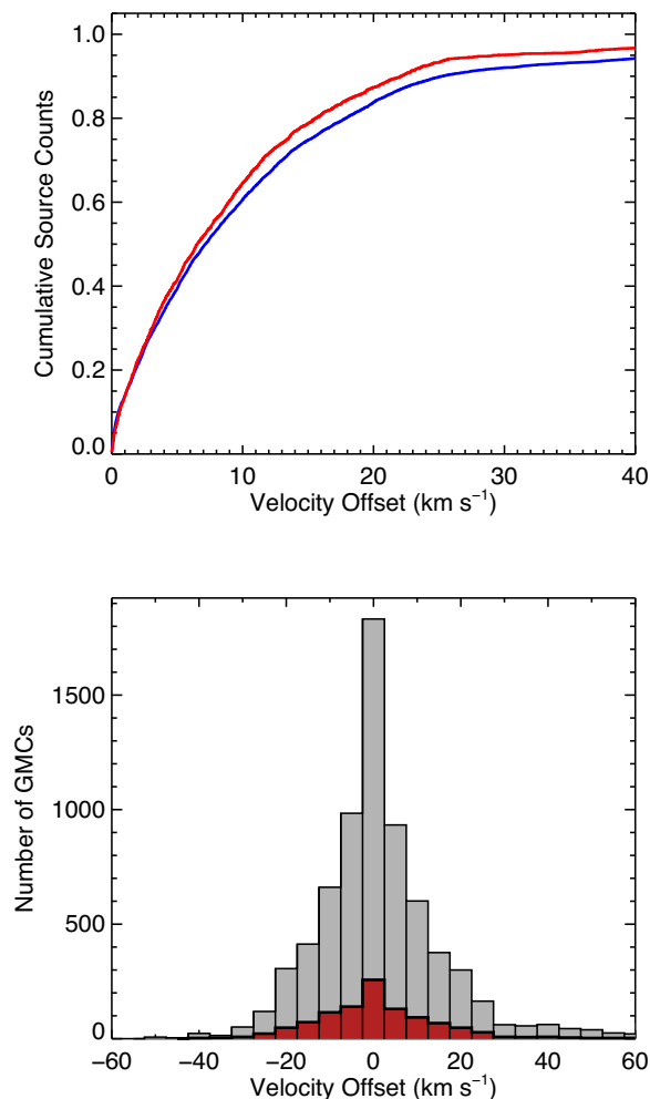
Figure 7. The upper panel shows the cumulative distribution of the absolute velocity separations of all ATLASGAL clumps (red curve) and SEDIGISM GMCs (blue curve) from their nearest spiral-arm locus in \ell - v space. The lower panel shows the frequency distribution of velocity differences of all GMCs (grey) and those associated with dense gas (red).
