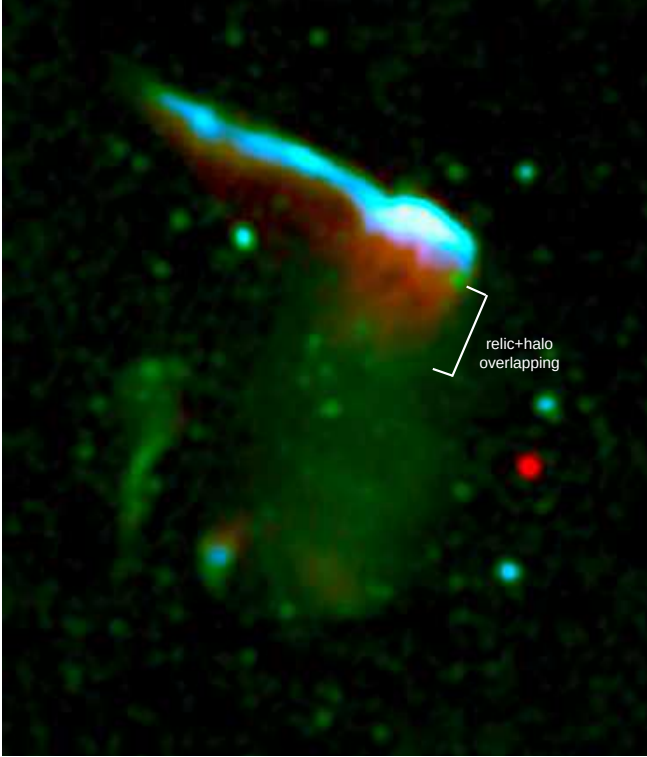
Fig. 5. Combined LOFAR (120-180 MHz), VLA L-band (1-2 GHz), and VLA S-band (2-4 GHz) image of the cluster at 15.7". The image clearly shows that B1 extends out of the relic and penetrates into the halo. As discussed in Sec 6.4, this is consistent with the superposition of the relic and the halo emission. The intensity in red, green, and blue shows the radio emission observed with the LOFAR, VLA L-band, and VLA S-band, respectively. The image properties are given in Table 2, IM10, IM13, and IM21.
