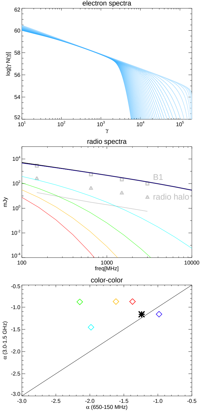
Fig. 14. Top panel: evolving spectrum of electrons accelerated by a \mathcal{M} = 3.8 shock and aging in a uniform 2.0 \mu\text{G} magnetic field (see text for other model parameters). Middle panel: evolving radio spectra as a function of time. The top black spectrum gives the integrated spectrum for the region corresponding to the entire B1 region, while the colored lines show the spectra within different 15'' \approx 54 kpc thick stripes perpendicular to the shock propagation axis. The additional gray symbols show the observed total integrated spectrum for B1 (top squares) and the radio halo (lower triangles), while the gray line gives the estimated contribution from the radio halo within each single 15'' stripe (assuming a flat brightness distribution). Bottom panel: color-color plot obtained by comparing the \alpha_{150 \text{ MHz}}^{650 \text{ MHz}} and \alpha_{1.5 \text{ GHz}}^{3 \text{ GHz}} spectral slopes within the stripes with corresponding colors, as in the central panel.
