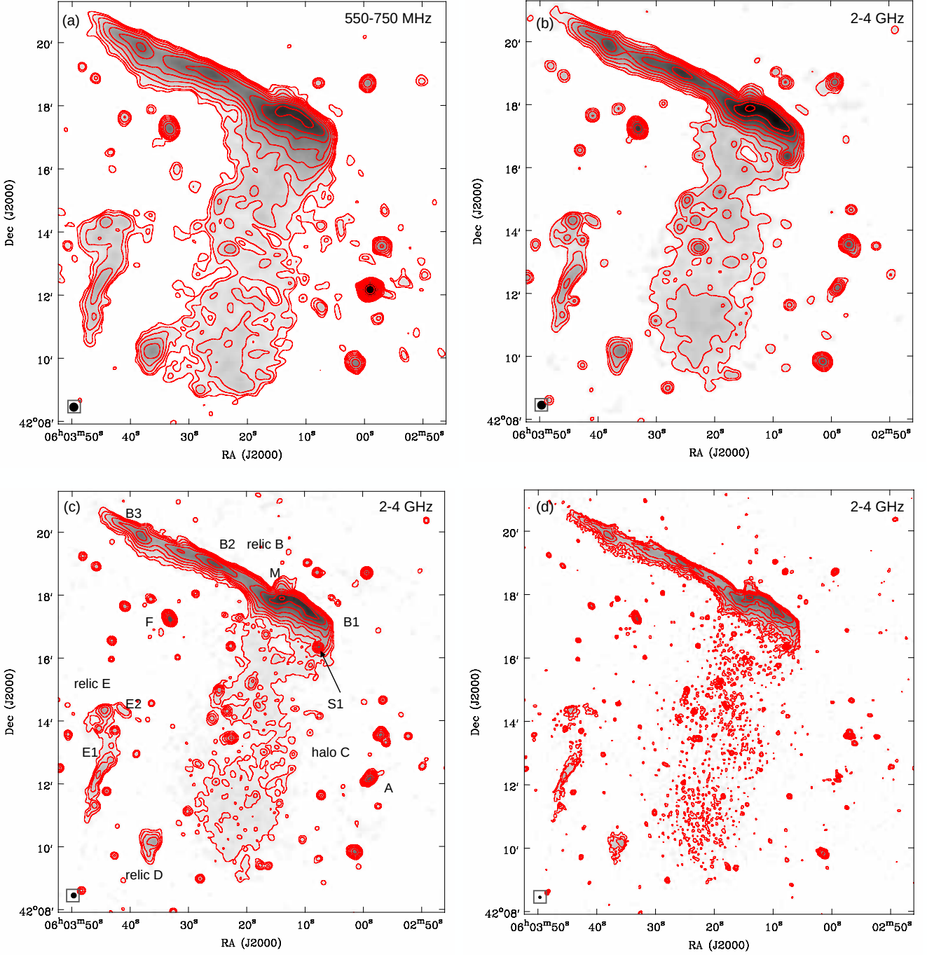
Fig. 1. uGMRT (550-750 MHz) and VLA S-band band images of 1RXSJ0603.3+4214. The known diffuse emission sources, namely the bright Toothbrush, the other two fainter relics to the west and the large elongated halo are recovered in both the uGMRT and the VLA (S-band) observations. The image properties are given in Table 2. Here, panel (a), (b), (c), and (d) correspond to IM17, IM9, IM8, and IM5, respectively. Contour levels are drawn at [1, 2, 4, 8, \dots] \times 4 \sigma_{\text{rms}} . The beam size are indicated in the bottom left corner of the image.
