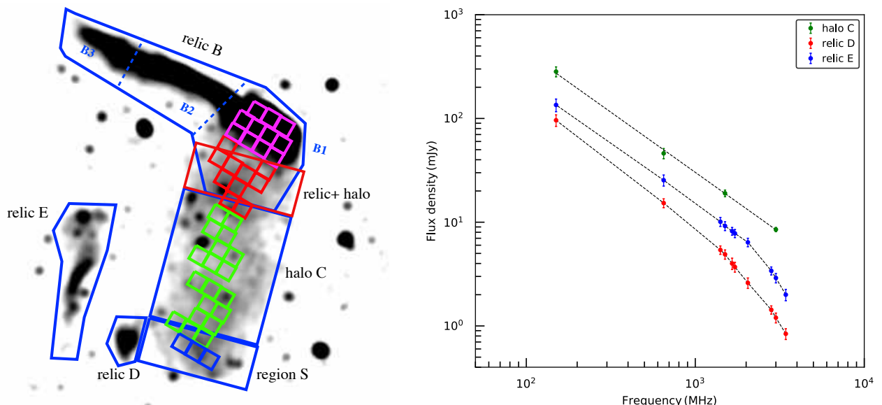
Fig. 7. Left: VLA 15'' resolution image depicting the regions where the integrated flux densities were measured. Right: Integrated spectra of the halo C and relics E and D. The spectrum of the halo C is well described by a single power-law spectrum. Relics E and D show spectral steepening beyond 1.5 GHz. The flux densities are measured from 15'' resolution images, created using uniform weighting with a uv-cut at 0.4 k \lambda .
