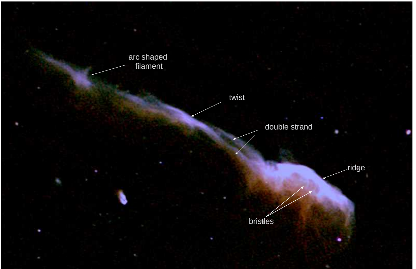
Fig. 4. Combined uGMRT (550-750 MHz), VLA L-band (1-2 GHz), and VLA S-band (2-4 GHz) image of the Toothbrush relic manifesting variety of small and large scale complex filamentary structures. The intensity in red, green, and blue shows the radio emission observed with the uGMRT, VLA L-band and VLA S-band, respectively. The colors reflect the local spectral index variations within the relic, although there is not a 1:1 match
