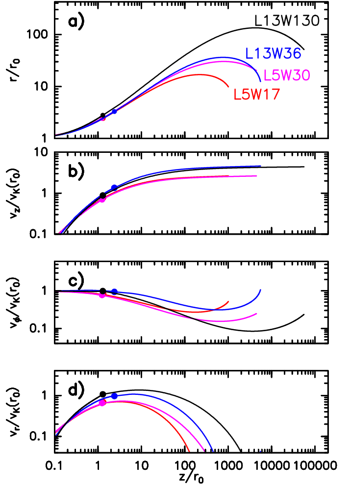
Fig. 2. Shape and kinematics of the streamlines as a function of vertical distance z above the disk midplane for the four computed MHD DW solutions in Table 1. a : cylindrical radius r , b : velocity along the jet axis V_z , c : azimuthal rotation velocity V_\phi , d : radial expansion velocity V_r . Filled dots indicate the Alfvén surface. Distances are scaled by the launch radius r_0 , and velocities by the Keplerian speed at r_0 , V_K(r_0) . Models are denoted as LxWy with x = \lambda_{\text{BP}} the magnetic lever arm parameter and y = \mathcal{W} = r_{\text{max}}/r_0 the widening factor (as defined in Eqs. (3) and (4) and listed in Table 1).
