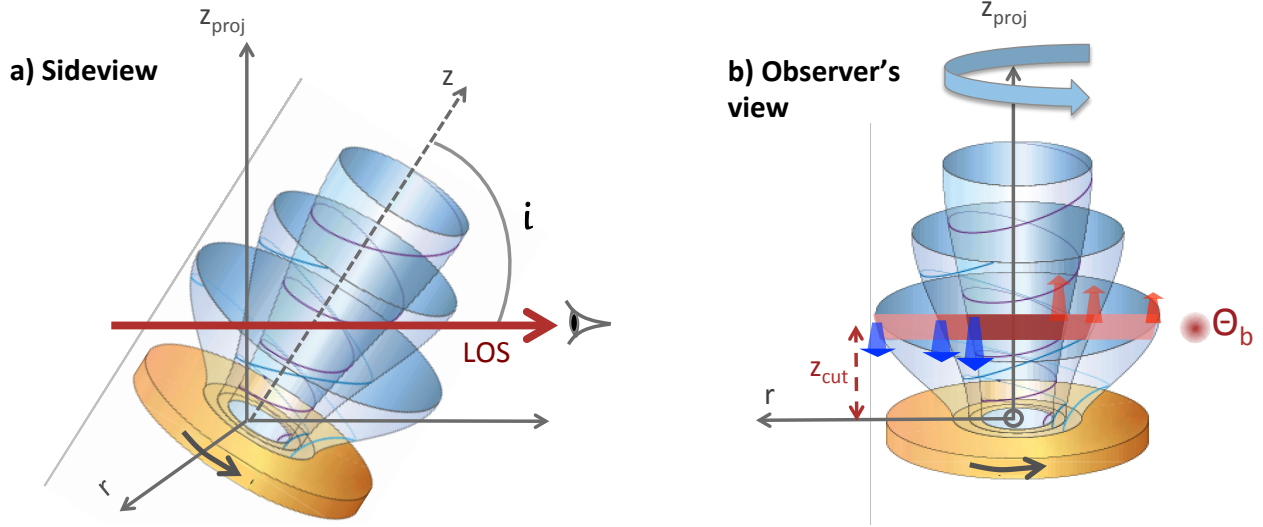
Fig. 3. a : definition of inclination angle i for our synthetic predictions in Sect. 3. b : sketch illustrating the construction of the transverse PV cut at projected altitude z_{\text{cut}} with a Gaussian beam \theta_b . Wind rotation induces different line-of-sight velocities at symmetric offsets +r and -r on either side of the jet axis, producing a detectable “tilt” in the PV cut (see Fig. 4). This projected velocity shift is used to estimate the rotation speed and specific angular momentum of the flow (see Sect. 3.2). Adapted from Ferreira (2001).
