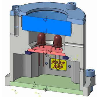
Figure 16. OPSE design, courtesy of LAM.
