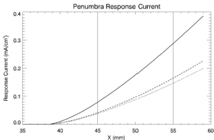
Figure 15: SPS response current in the penumbra on the entrance pupil plane as a function of the distance from the telescope optical axis.
