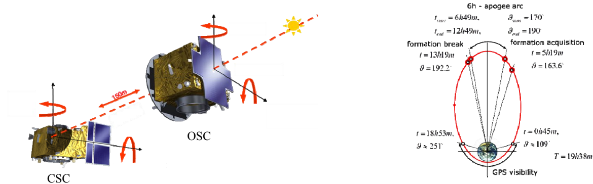
Figure 1: PROBA-3 formation flying overview and orbit.
