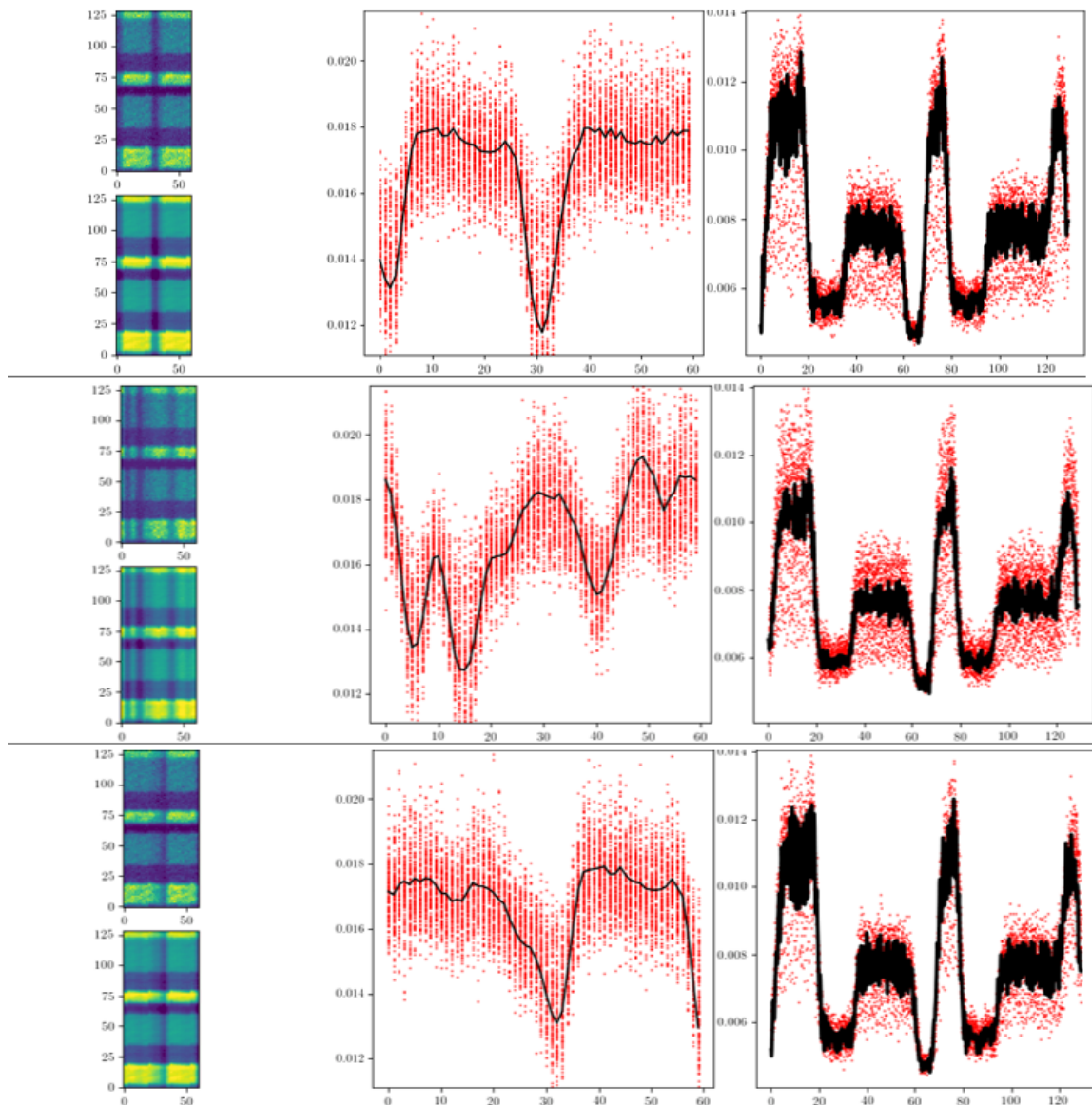
Figure 16. Order tracing along spectral direction of the order 146 of HIRES Z band. Left upper panel : RAW data. Left bottom panel : reconstructed surface. Right panels : Extracted scientific spectrum and illumination profile of the fiber-slit.
