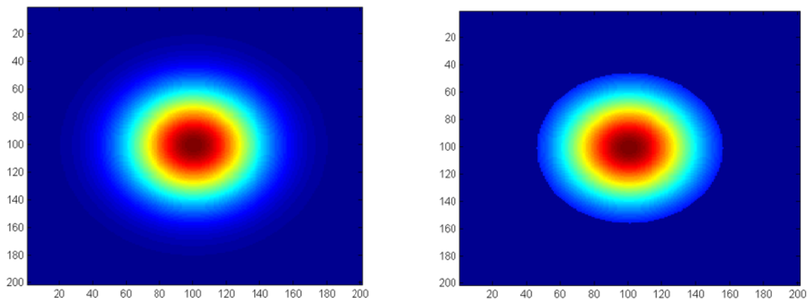
Figure 8. Front-End focal plane. Left panel: the telescope focal plane image is convolved with the estimated FE PSF of 0.025 arcsec. Right panel: Portion of the FE unit focal plane light distribution that feeds the dicing unit aperture.
