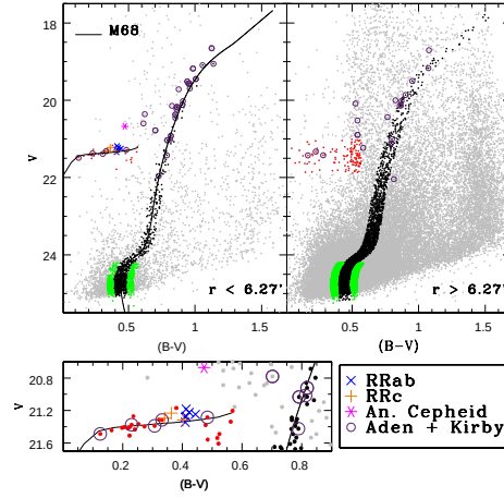
Fig. 1. Top left: V, B - V CMD of the Hercules UFD, drawn from all the stellar-like objects (grey dots) within the galaxy half-light radius ( r_h \simeq 6.27' , Sand et al. 2009). The black line is the ridgeline of the Galactic GC M 68. Black and green dots are stars respectively within \pm 0.05 mag in B - V and from \pm 0.05 to \pm 0.1 mag from the ridgelines of M 68. Red dots are non-variable stars in the HB region. The fundamental-mode (RRab) and the first-overtone (RRc) RR Lyrae stars are marked by blue crosses and orange plus signs, respectively, the Anomalous Cepheid by a magenta asterisk. Open violet circles mark member stars of the Hercules UFD identified spectroscopically by Kirby et al. (2008) and spectrophotometrically by Adén et al. (2009). Top Right: V, B - V CMD of all the stellar-like objects outside the half light radius. (Symbols and color-coding are as in the top left panel). Bottom: An enlargement of the HB region of the CMD in the top left panel.
