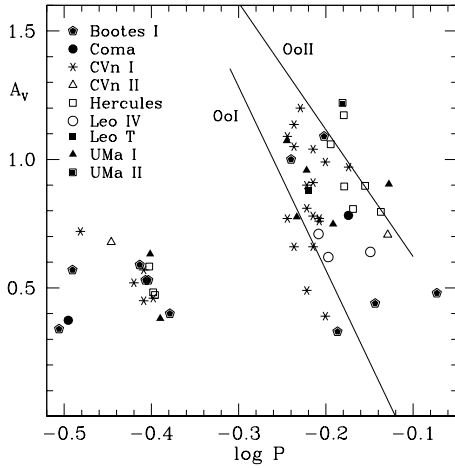
Fig. 2. V-band period-amplitude diagram of the RR Lyrae stars in the UFDs studied so far for variability. Solid lines are the positions of the Oo I and II Galactic GCs, from Clement & Rowe (2000).
