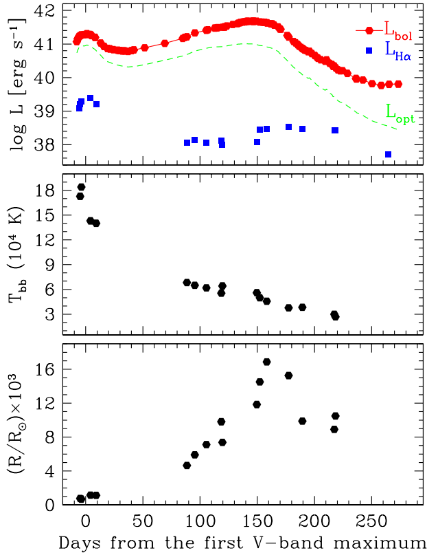
Fig. 12. Evolution of the bolometric, optical ( BVRI ) and \text{H}\alpha luminosities ( top panel ), continuum temperature ( middle panel ) and photospheric radius ( bottom panel ) in our spectra of NGC 4490–2011OT1. A conservative error of 500 K is estimated for the blackbody continuum temperature.
