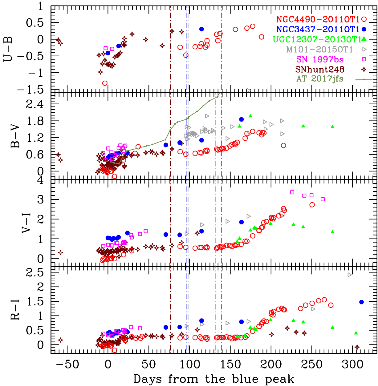
Fig. 4. Colour evolution for our sample of LRNe. The phase is in days from the first V band maximum. For UGC 12307–2013OT1, we tentatively adopted JD = 2 456 350 as epoch of the first peak. The dot-dashed vertical lines (plotted maintaining the same colour codes as the symbols) mark the epochs of the red maximum for the different objects. In SN 1997bs, the red maximum was not observed. The B - V colour curve of AT 2017jfs (Pastorello et al. 2019) is also shown as a comparison (solid line).
