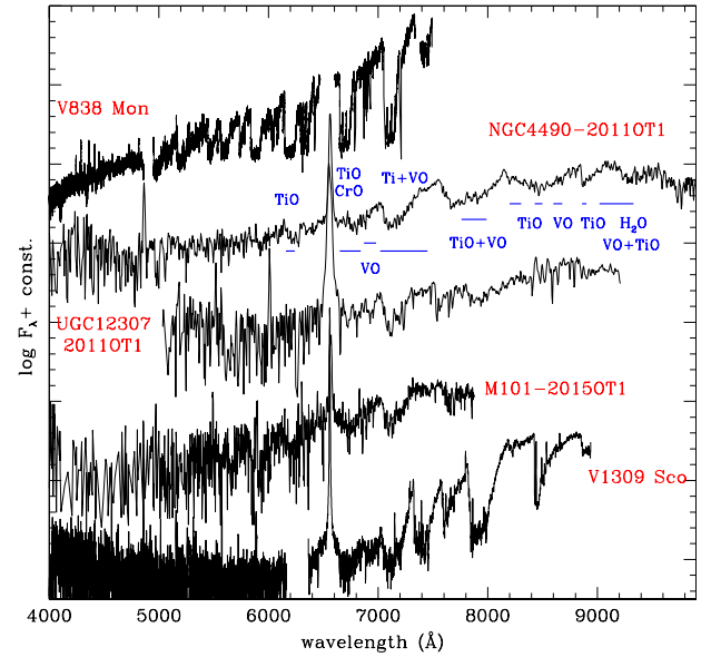
Fig. 13. Detection of molecules in late spectra of NGC 4490–2011OT1, UGC 12307–2013OT1 and M 101–2015OT1 (Blagorodnova et al. 2017), and comparison with late spectra of RNe V838 Mon (Kamiński et al. 2009) and V1309 Sco (Mason et al. 2010). \text{H}\alpha and \text{H}\beta are excised in the spectrum of V838 Mon to emphasize the broad molecular absorption bands.
