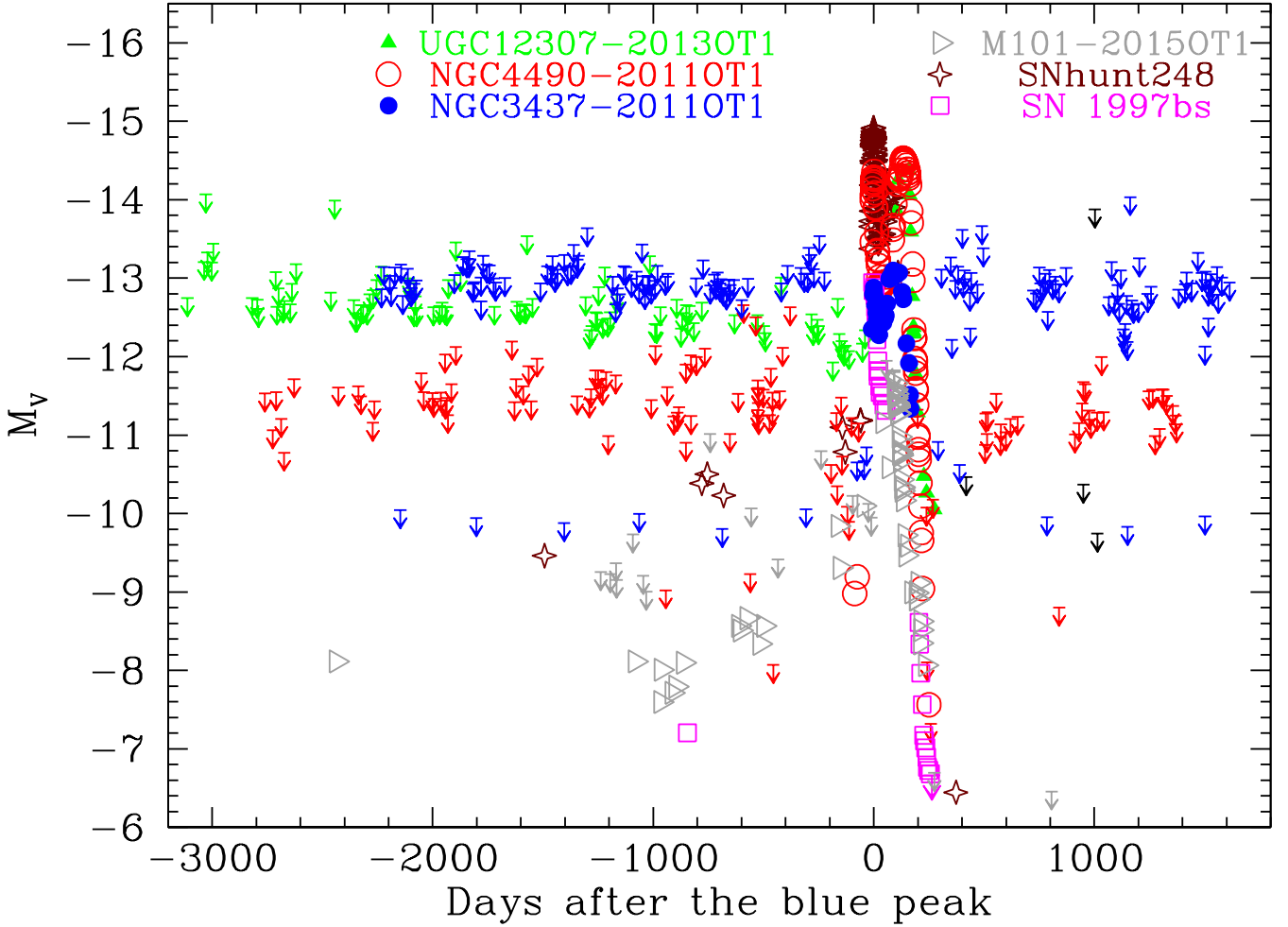
Fig. 6. Long-term photometric monitoring (specifically, V-band absolute magnitudes) for extra-Galactic LRNe discussed in this paper, covering about a decade of their evolution. Pre- and post-discovery detection limits are indicated with “down-arrow” symbols. The phase is in days from the first (blue) peak in the V band. The absolute light curves of LRN outbursts are compared in detail in Sect. 5.2.
