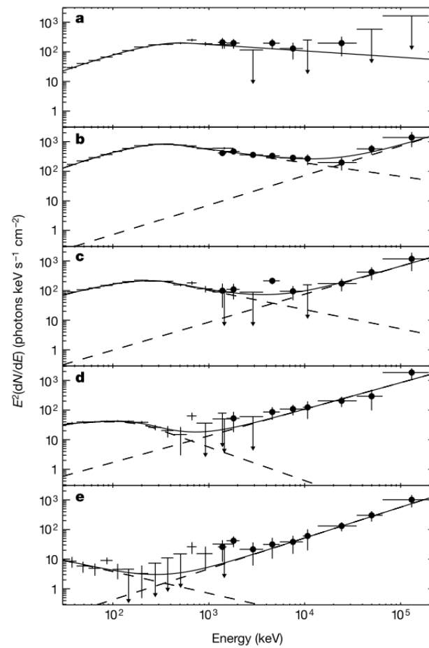
Figure 1. Gamma-ray spectra of GRB 941017. Five time intervals are shown in five separated panels, from the beginning of the prompt phase to more than 200 s (panel a : 18–14 s; b : 14–47 s; c : 47–80 s; d : 80–113 s; e : 113–211 s). Crosses and filled circles show BATSE and EGRET data, respectively. The model fit (solid curve) is composed by a superposition of a smoothly broken PL (Band model) and a PL function. Two distinct spectral component are clearly present, except in the first time interval. From [35].
