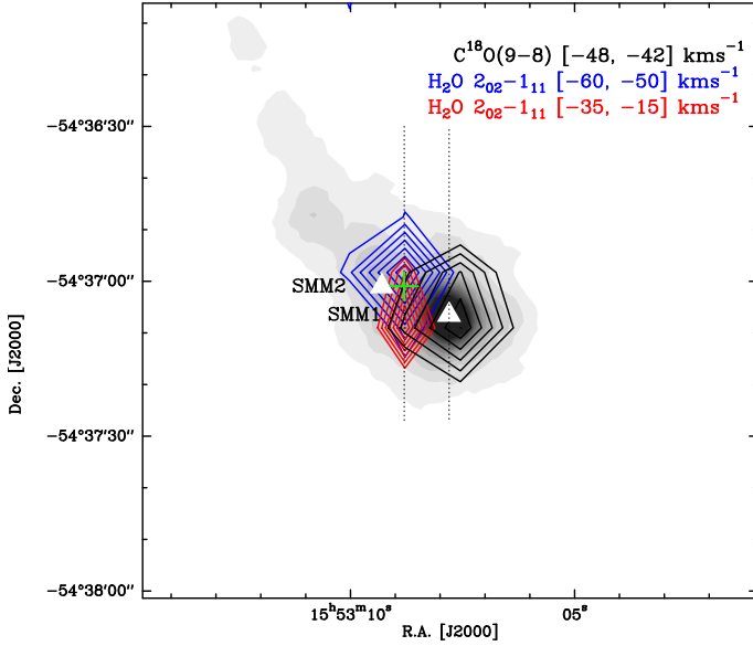
Fig. 7. Integrated intensity map of the p-H 2 O 2 02 -1 11 line in the blue- ([−60, −50] km s −1 , blue contours from 30% of the peak emission in steps of 10%) and redshifted ([−35, −15] km s −1 , red contours from 30% of the peak emission in steps of 10%) velocity ranges toward the IRDC region. The gray contours represent the integrated intensity of C 18 O(9–8) ([−48, −42] km s −1 , from 50% of the peak emission in steps of 10%). The white triangles mark SMM1 and SMM2, the green cross the position observed in the single-pointing HIFI observations (labeled as outflow in Fig. 8.) The dotted lines outline the cuts used to derive the P-V diagrams discussed in Sect. 3.2.1).
