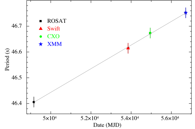
Fig. 7. Long-term spin down of CXOU J225355.1+624336 from ROSAT, Swift , Chandra , and XMM-Newton measurements (updated from Esposito et al. 2013). We attributed an error of 0.02 s to each point, reflecting the uncertainty due to the orbital motion (see Esposito et al. 2013 for details). The grey line indicates the best-fitting period derivative, \dot{P} \approx 5.3 \times 10^{-10} \text{ s s}^{-1} .
