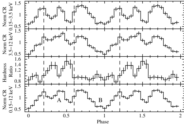
Fig. 2. Pulse profile and HR of CXOU J225355.1+624336 in the energy ranges 0.15–3.5, 3.5–12, and 0.15–12 keV. The dashed vertical lines delimit the two phase intervals, A and B (corresponding, respectively, to the maximum and minimum of the HR), selected for the phase-resolved spectral analysis.
