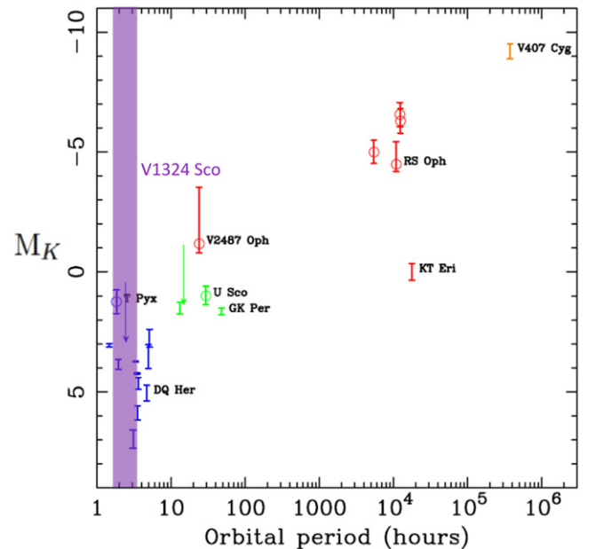
Figure 5. Plot showing the distribution of novae as a function of absolute K -band magnitude and binary orbital period, taken from Darnley et al. (2012). V1324 Sco is marked as the purple transparent line, indicating that we know the period \sim 1.6 hr, but we cannot place a limit on the absolute K -band magnitude. The width of the purple line corresponds to the fact that the period could either be 1.6 or 3.2 hr. The colors on the plot correspond to the luminosity class of the secondary: blue is main sequence, green is sub-giant, and red is giant.
