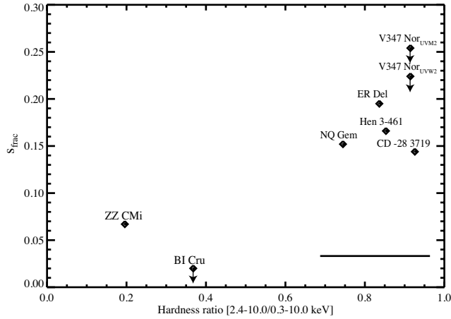
Figure 4: Fractional rms amplitude of flickering ( S_{\text{frac}} ) vs. hardness ratio in X-rays. Objects with harder X-ray emission tend to have more intense UV flickering. Downward arrows indicate upper limits. The average error bar is shown at the bottom-right corner [from 115]
