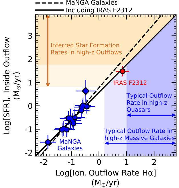
Figure 10. Star formation rate inside the outflow as a function of ionized gas mass outflow rate inferred from the \text{H}\alpha . Blue symbols are star forming outflows in local MaNGA galaxies studied in this paper. The red symbol indicates the star forming outflow previously detected in IRAS F23128-5919 (Maiolino et al. 2017). The dashed line shows the fit to the MaNGA outflows presented in this paper (blue points). The solid line is the linear fit including IRAS F23128-5919 (Eq. 2). The blue shaded regions indicate the ionized outflow rate inferred for high- z massive galaxies and quasars. The orange shaded regions indicates the star formation rate inside these distant galactic outflows if they follow the same correlation observed locally.
