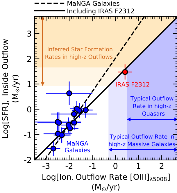
Figure 11. As Figure 10, but where the ionized outflow rate is now inferred from the broad component of the [OIII] line.
