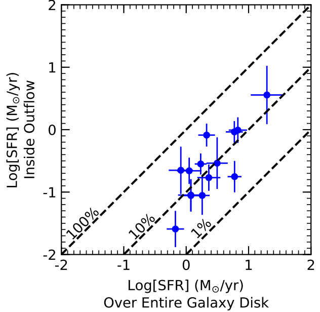
Figure 8. Star formation rate inside the outflow as a function of total star formation rate in the disc of the host galaxy.
