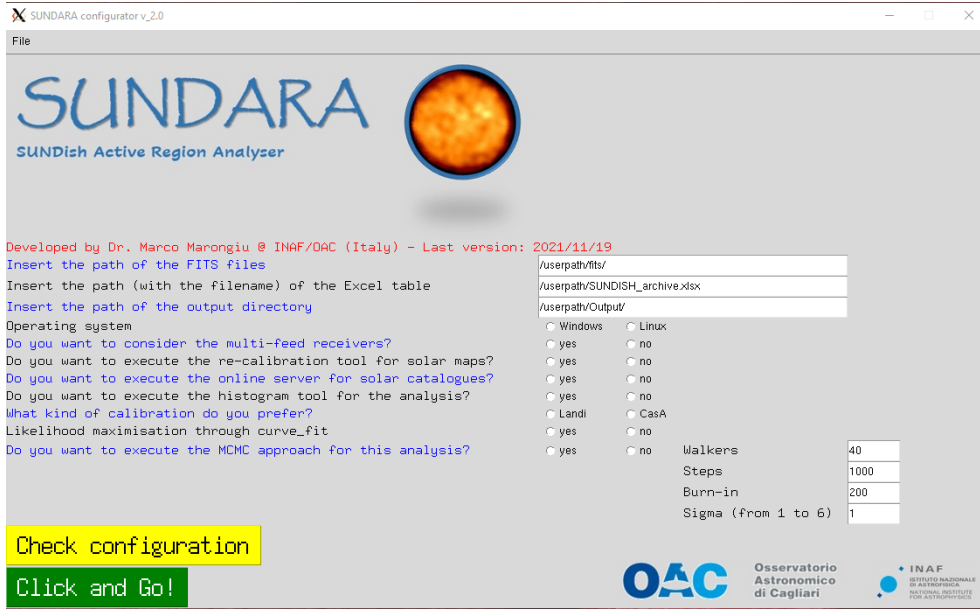
Figure 4: Widget of the SUNDARA Python Package. The user must compile all the boxes before clicking the “Click and Go!” button, and hence executing SUNDARA.
