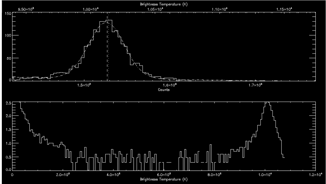
Figure 3: Example of histogram of pixel values in the image, in linear scale, produced by the self-calibration process with SDI. (top) - Zoomed part of this distribution, well fitted by a Gaussian (dashed line), whose peak corresponds to the RMS value of the QS brightness temperature, and the width is connected with the solar activity. (bottom) - Complete histogram of the brightness temperature distribution. The tail of the quasi-Gaussian distribution at low brightness temperature in the histogram is due to the brightness gradient of the corona.
