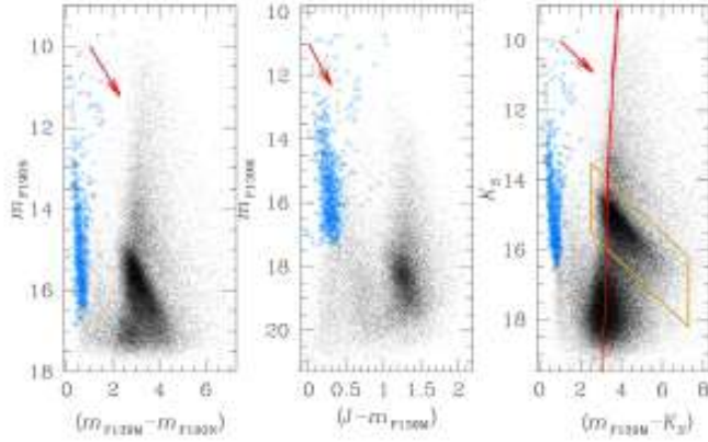
Figure 7. CMDs based on the WFC3/IR data. Left-hand panel: m_{F139M} versus (m_{F139M} - m_{F139N}) CMD. Middle panel: m_{F139M} versus (J - m_{F139M}) CMD. Right-hand panel: K_S versus (m_{F139M} - K_S) CMD. Blue open circles depict stars in common with the Gaia -DR2 catalogue. In each CMD, the direction of the reddening vector is indicated by a red arrow. The reddening vector is computed by assuming an arbitrary extinction A_{F139M} in each plot and the extinction index \alpha = 2.3 of Noguera-Lara et al. (2018). A PARSEC isochrone for 10-Gyr-old stars with [\text{Fe}/\text{H}] = -0.16 at 8.2 kpc from the Sun representing the Bulge population is fitted by eye as reference in the rightmost panel. The gold rectangle marks the location of the Bulge red clump.
