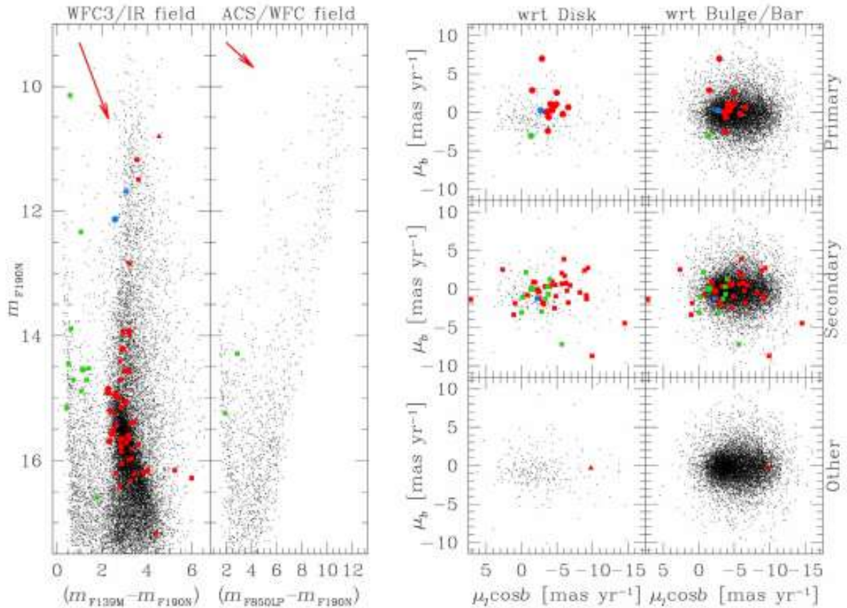
Figure 22. Similar to Fig. 14 but for candidate MSs.
