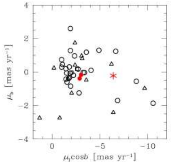
Figure 17. VPDs of the PMs of the confirmed MSs (black points). The red star marks the PM of Sgr A*, while the two red points indicate the PMs of the Arches and Quintuplet clusters. As in Fig. 14, circles, squares, and triangles represent MSs in the Primary, Secondary, and Other samples, respectively.
