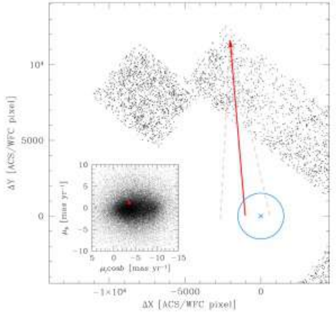
Figure 18. PM of the MS #20612 relative to Sgr A*. The red solid arrow starts at the time of the closest approach (see Table 3) and ends at the current position of the star. Pink dashed arrows define the confidence region. The blue circle has a radius of \sim 1.26 arcmin and is centred on the position of Sgr A* (blue cross). The absolute PM of the source is shown in the VPD in the inset. Only 25 per cent of the bright sources are shown. North is up and east is to the left.
