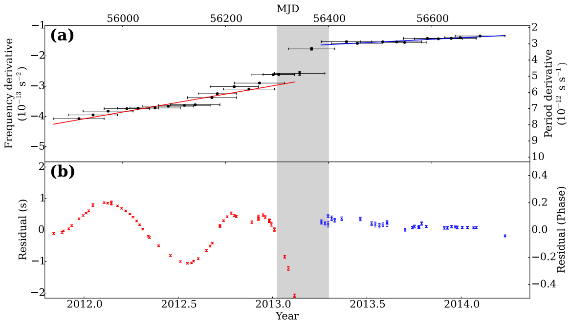
Figure 4. The rotation of PSR J1622–4950. Red and blue lines and points correspond to two simple ( \nu , \dot{\nu} , \ddot{\nu} ) timing solutions. (a) Frequency derivative. Black points represent short-term measurements of the frequency derivative (see Section 3.3). (b) Timing residuals for the two timing solutions (Table 1). The gray bar marks the period between MJD 56300 and MJD 56400 in order to illustrate the correlated behavior between the spin-down, flux density (Figure 3), and pulse profile evolution (Figure 2) at that time.
