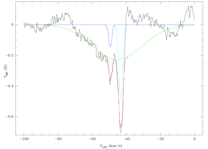
Fig. 17. Spectra of p\text{-H}_2^{18}\text{O } 1_{11}-0_{00} line (in black) showing the different Gaussian components used to fit the line (red = green+blue+purple).
