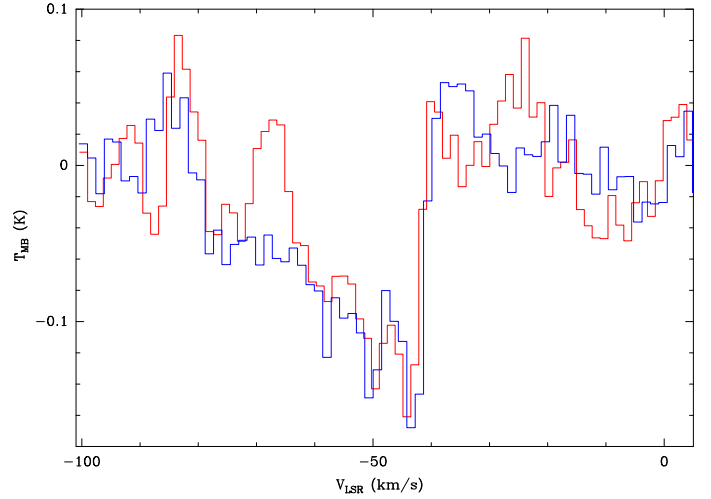
Fig. 16. Spectra of o\text{-H}_2^{17}\text{O } 2_{12}-1_{01} ( \times 0.3 , in blue) line overplotted on the p\text{-H}_2^{17}\text{O } 1_{11}-0_{00} spectrum (in red). The spectra have been smoothed to 1.4 \text{ km s}^{-1} .
