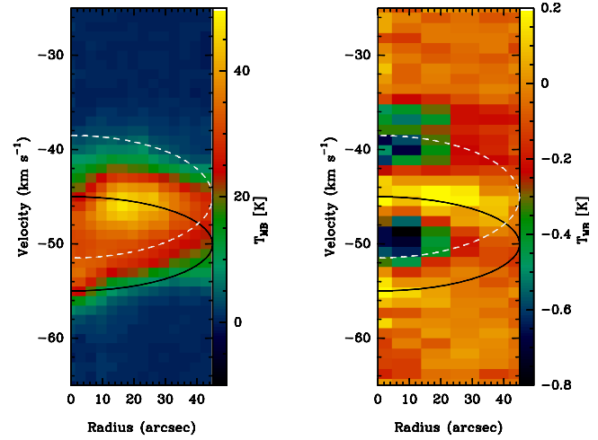
Fig. 10. ( r-v ) diagrams of the HII region G327.3–0.5 obtained from the 12 CO(6–5) ( left ) and from the 1 11 –0 00 –p H 2 O ( right ) data cubes. The radius axis is the distance to the shell expansion center, chosen to be the peak of the cm continuum emission. The black solid half-ellipse represents an ideal shell in ( r-v ) diagram with an expansion velocity of 5 km s –1 centered on –50 km s –1 , the dashed white half-ellipse an ideal shell with an expansion velocity of 6.5 km s –1 centered on –45 km s –1 .
