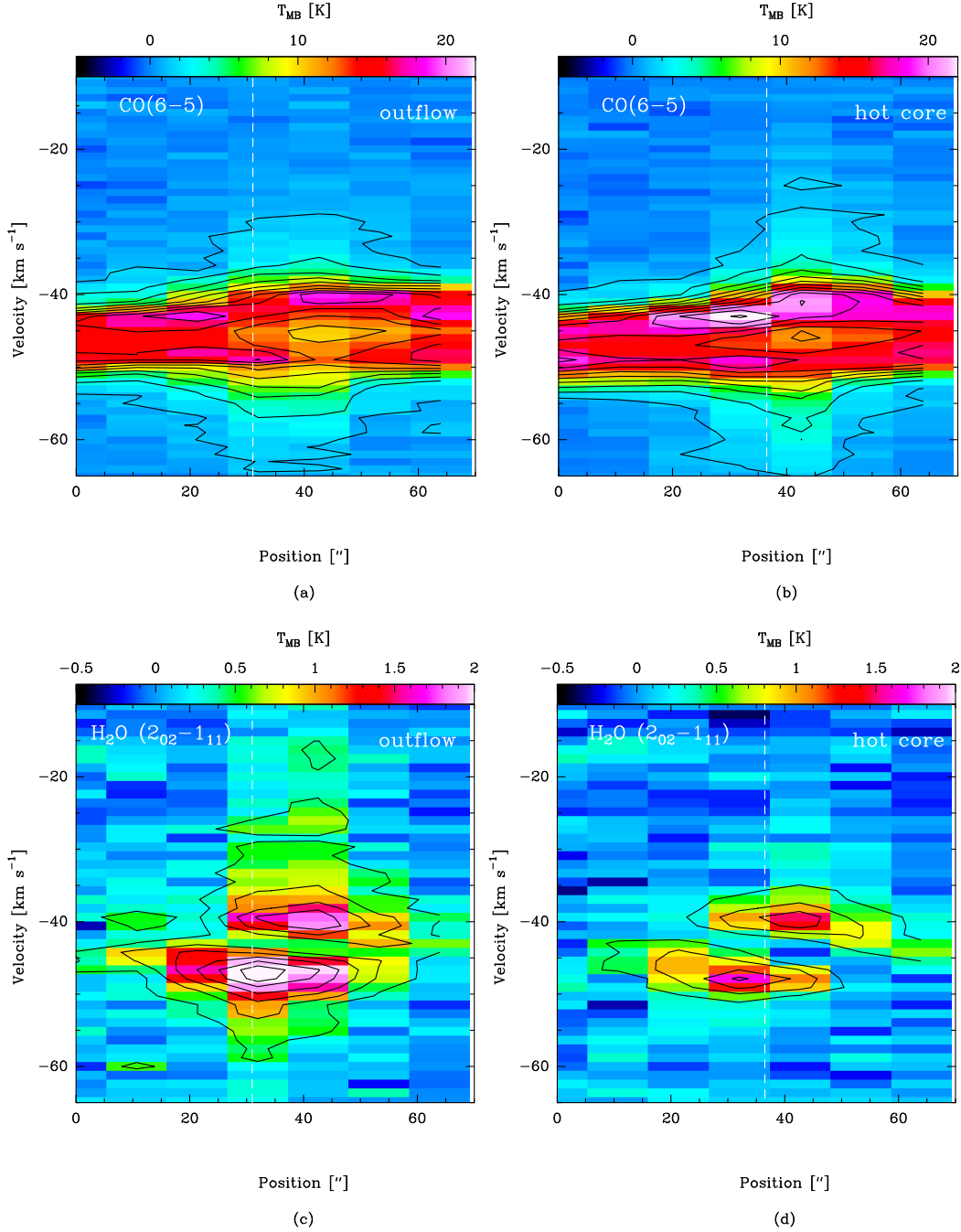
Fig. 8. Top: color scale and contours show the P-V diagram of the CO(6–5) transition computed along a vertical cut passing through the outflow a) and the hot core position b) . Bottom: color scale and contours show the P-V diagram of the 2_{02}-1_{11} H 2 O line computed along a vertical cut passing through the outflow c) and the hot core position d) . The cut through the outflow position is from \alpha_{J2000} = 15^{\text{h}}53^{\text{m}}08^{\text{s}}.8, \delta_{J2000} = -54^{\circ}36'30'' to \alpha_{J2000} = 15^{\text{h}}53^{\text{m}}08^{\text{s}}.8, \delta_{J2000} = -54^{\circ}37'27'' , the cut through the hot core from \alpha_{J2000} = 15^{\text{h}}53^{\text{m}}07^{\text{s}}.8, \delta_{J2000} = -54^{\circ}36'30'' to \alpha_{J2000} = 15^{\text{h}}53^{\text{m}}07^{\text{s}}.8, \delta_{J2000} = -54^{\circ}37'27'' . Offset positions increase along the direction of the cuts. Contours are from 3\sigma in steps of 3\sigma for H 2 O, and in steps of 5\sigma for CO.
