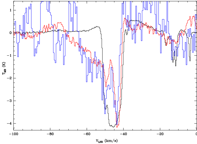
Fig. 15. Spectra of p\text{-H}_2^{18}\text{O } 1_{11}-0_{00} ( \times 6.2 , in red) and p\text{-H}_2^{17}\text{O } 1_{11}-0_{00} ( \times 21 , in blue) lines overplotted on the p\text{-H}_2\text{O } 1_{11}-0_{00} spectrum (in black). The spectra have been smoothed to 0.3 \text{ km s}^{-1} ( 1.4 \text{ km s}^{-1} for the \text{H}_2^{17}\text{O} spectrum).
