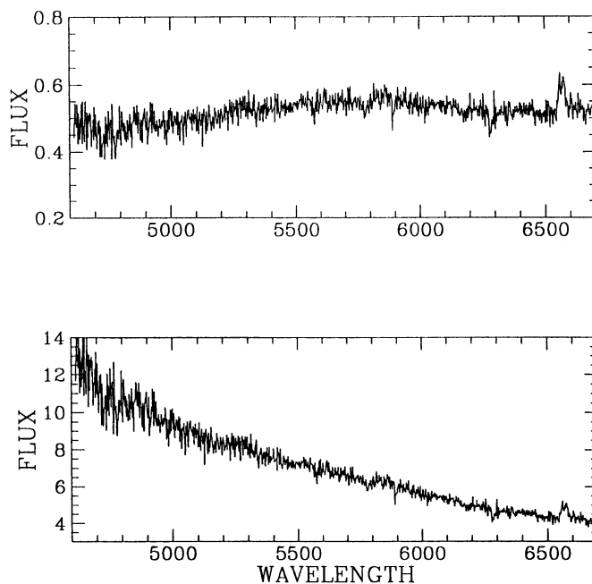
Fig. 4. Upper panel: observed spectrum of nova Oph 1993. Lower panel: spectrum of nova Oph 1993 after the correction for interstellar absorption (ordinate: 10^{-15} erg cm ^{-2} s ^{-1} Å ^{-1} ). We have assumed E(B-V)=0.9
