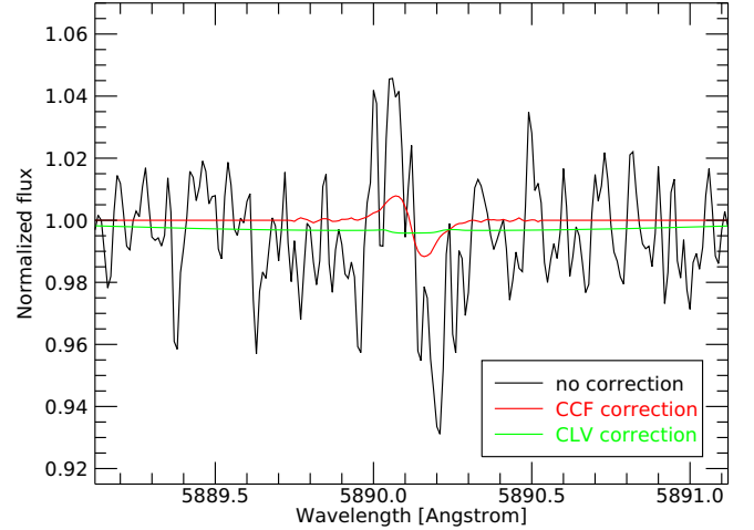
Fig. 6. Example of a single transmission spectrum of HD 189733b, zoomed on the sodium D2 line, with the corrections of CLV and RM overimposed. The RM correction in particular looks underestimated, as discussed in Sect. 5.
