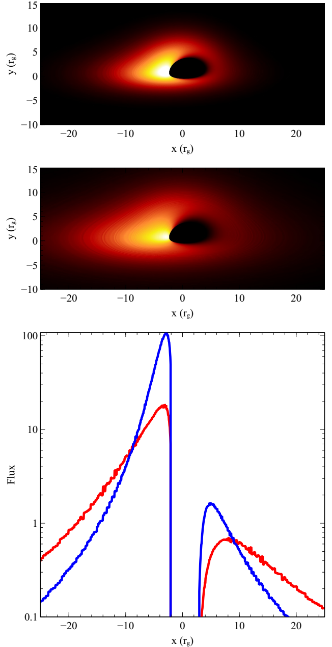
Figure 3. Top: Intensity-weighted image of a disc irradiated by a corona at height h = 4r_g , appropriate for the low-flux state. The colour table is logarithmic spanning a range of 1000 from white to dark red. x and y are in the image plane. Centre: Similar plot for h = 10r_g to represent the high flux state. Bottom: Flux profiles along a midplane cut. Blue line is h = 4r_g lampost; red line is h = 10r_g .
