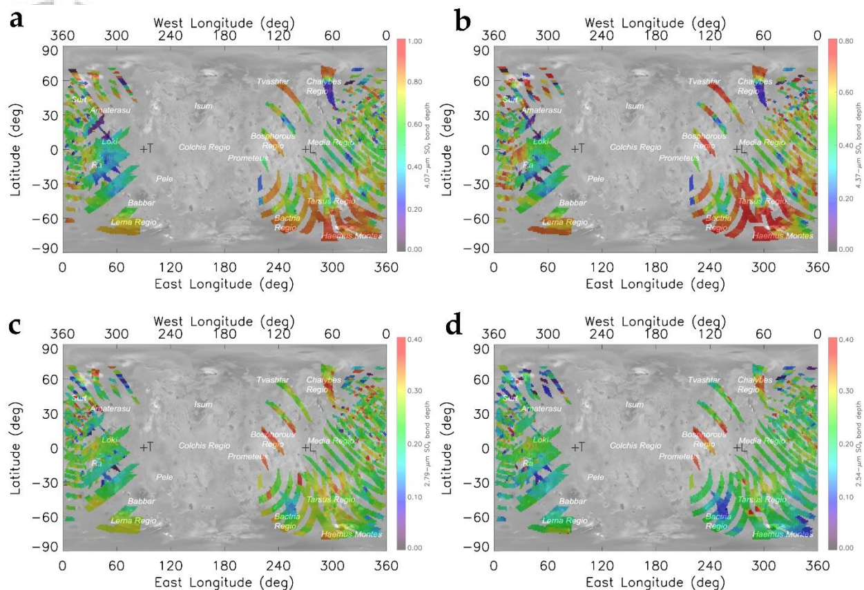
Figure 4. Spatial distribution of the depth of the strongest absorption bands diagnostic of SO 2 frost, revealed between 2.5 and 4.5 \mu\text{m} . a. Map of band depth for the main SO 2 band, centered at 4.07 \mu\text{m} . b. Map of band depth for the 4.37- \mu\text{m} signature. c. Map of band depth for the 2.79- \mu\text{m} absorption. d. Map of band depth for the 2.54- \mu\text{m} feature. The maps derived from the weighted averages of JIRAM-derived band depths are transparently superimposed on an optical mosaic of the Io surface, to facilitate association with some of the major geologic formations. Color bars have different ranges in different panels, because the absorption bands at 4.07 \mu\text{m} and 4.37 are much stronger than the bands at 2.79 and 2.54 \mu\text{m} . In all maps presented in this figure and in the following ones, the horizontal axes express both east and west longitudes, so as to enable a quick comparison with past results, which used west longitudes, but also facilitate a comparison with the data that will be acquired by future space missions such as JUICE and Europa Clipper, which may favor eastward longitudes. The “+T” and “+L” symbols mark the apex of the trailing and leading hemispheres, respectively.
