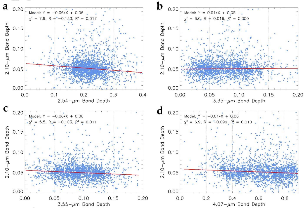
Figure 8. Scatterplots related to the BD values measured for: 2.10 μm band vs. 2.54 μm band (panel a ), 2.10 μm band vs. 3.35 μm band (panel b ), 2.10 μm band vs. 3.55 μm band (panel c ), and 2.10 μm band vs. 4.07 μm band (panel d ). In each scatterplot, a linear fit model (red line) is superimposed on the distribution. The values of the chi-square ( \chi^2 ), the Pearson correlation coefficient ( R ), and the coefficient of determination (i.e., the squared correlation coefficient R^2 ) coming from the linear fit are also reported. These scatterplots are meant to evaluate whether and how much the very weak band centered at 2.1 μm, usually attributed to sulfur dioxide, is related to other bands of the same compound located at longer wavelengths. In doing so, and to avoid that our results be substantially affected by grain size effects, we consider not only the strongest band centered at 4.07 μm, but also the weak band at 2.54 μm and those, even weaker, centered at 3.35 and 3.55 μm, whose relative strength is comparable to that of the 2.1-μm band.
