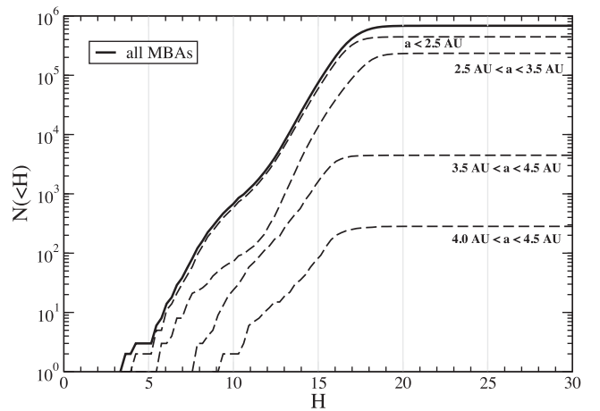
Figure F4. Cumulative distribution of the absolute magnitudes of the Main Belt asteroids (data from Minor Planet Center, March 2016). The bold line represents the distribution of all Main Belt asteroids, while long-dashed lines are the distributions for some sub-groups, selected according to different intervals of the semi-major axis.
