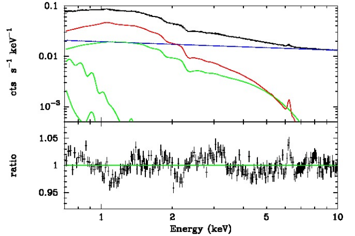
Fig. B.1. Top panel: simulated data and best fit model when making use of the full spectral range. The source is shown in red, the sky fore- and background in green, and the instrumental background in blue. Bottom panel: residuals in the form of a data over model ratio. All residuals are below 5%, and are due to differences in the effective area and foreground parameters used in the simulation with respect to those adopted for the fit. We note how the low abundance value forced by the data around the Fe L-shell results in residuals around the Fe K\alpha line.
