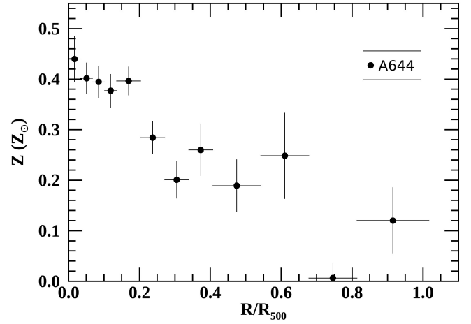
Fig. 2. Iron abundance profile for A644 as a function of R/R_{500} , derived with standard X-COP analysis (see Sect. 2.2).
