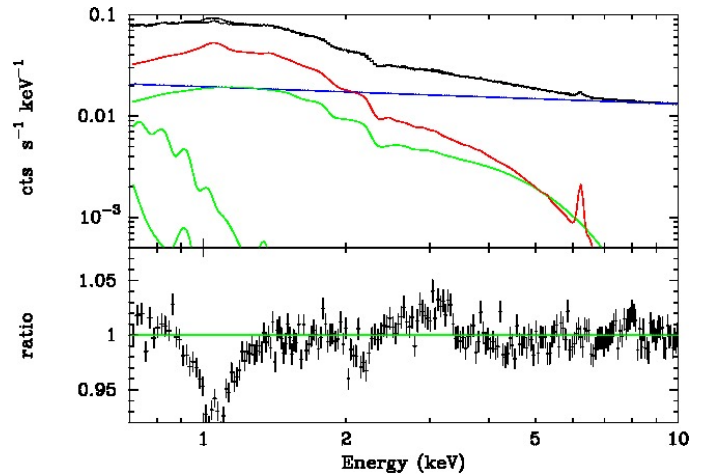
Fig. B.2. Same as for Fig. B.1 except that the L-shell range (0.9–1.3 keV) is excluded from fitting. We note how the residuals around the Fe K\alpha line are no longer present.
