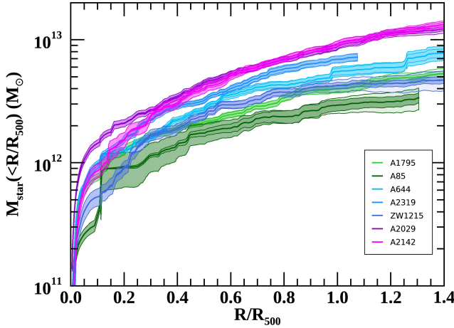
Fig. 16. Cumulative stellar mass profiles. Dark shades are statistical uncertainties, faint shades are cosmic variance uncertainties.
