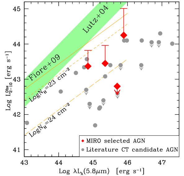
Fig. 3. \text{Log}(L_{\text{X}}^{\text{Obs}}) vs. \text{Log}(L_{5.8\mu\text{m}}) for several CT candidates. Grey circles represent literature CT candidate AGN (see Lanzuisi et al. 2015a, for more details). Red diamonds represent our MIRO targets; intrinsic X-ray luminosities of the X-ray detected objects are also indicated with upper bars. The green shaded area is the relation of Lutz et al. (2004) for a sample of low-redshift, unobscured AGN. The orange solid line is the relation for high-redshift unobscured AGN (Fiore et al. 2009), while the dashed and long dashed lines are the expected relation for a 10^{23} \text{ cm}^{-2} and 10^{24} \text{ cm}^{-2} absorber.
