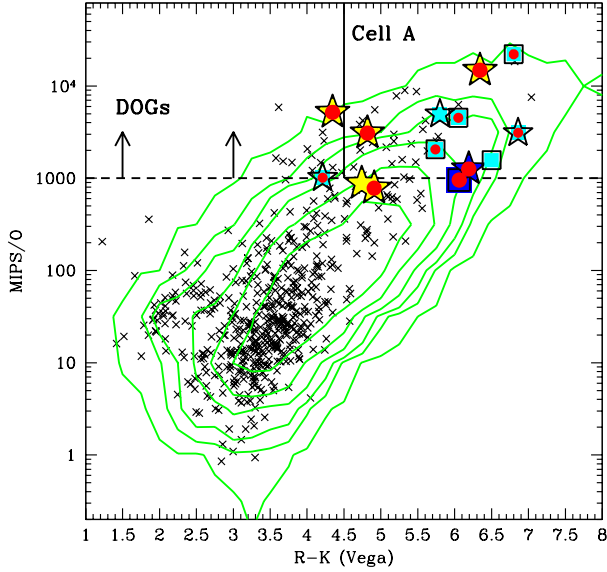
Fig. 1. f_{24\mu\text{m}}/f_R as a function of R - K colour for all the COSMOS 24\mu\text{m} sources associated with the optical and K -band counterparts (green isodensity contours). Black crosses represent the 1 mJy flux-limited sample. Yellow stars denote the five objects observed with SINFONI; cyan stars and squares denote Melbourne et al. (2011) and Brand et al. (2007) targets, respectively (two targets present in both samples are indicated with stars); blue symbols denote the Perna et al. (2015) targets. Star and square symbols indicate IFU and long-slit observations, respectively. Sources marked with red circles are also detected in the 1 mJy flux limited sample and are those considered for the analysis. The box delimited by a vertical solid line and horizontal dashed line marks the region proposed in Fiore et al. (2009) to select CT AGN (Cell A). The horizontal dashed line sets the criterion for the selection of DOGs.
