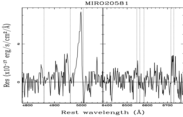
Fig. 7. MRO20581 residuals in the [OIII] and H \alpha range obtained by fitting the observed lines with only NLR and BLR components. (See Sect. 5; to be compared to Panel a of Fig. 6.)
