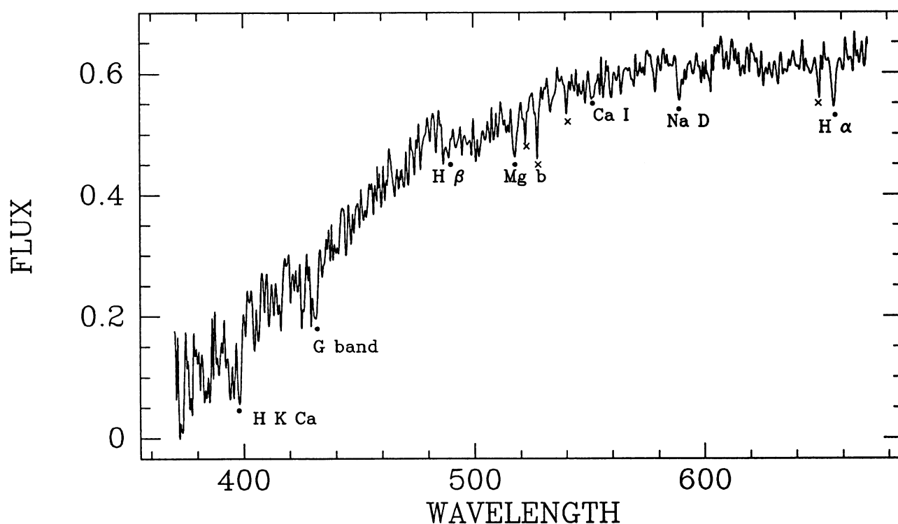
Fig. 1. The spectrum of the gravitational microlensing candidate. Ordinate are units of 10^{-16} \text{ erg s}^{-1} \text{ cm}^{-2} \text{ nm}^{-1} . Features marked with 'x' represent cosmic rays and/or artifacts not corrected. Dots represent real features.
