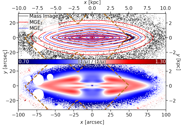
Fig. A.1. Mass-density MGE for FCC 153. Top: contours of the projected mass density (black), the mass density MGE Σ (red), and the surface brightness MGE μ (blue). Bottom: ratio between the mass and surface-brightness models, showing the structural differences. This panel is normalised by the average M_{\star}/L such that values of 1.0 (white) are consistent with the assumption of a spatially-constant M_{\star}/L , and any deviations are percentages in stellar mass. The outline of the MUSE mosaic is shown in dashed brown.
