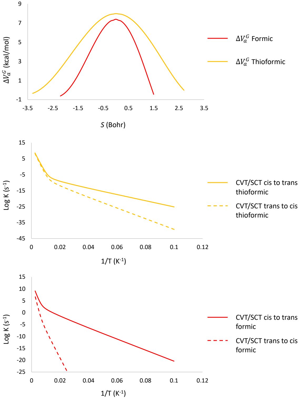
Fig. 3. Relative V_a^G potentials with respect the cis isomers in \text{kcal mol}^{-1} . Arrhenius plots for the cis to trans (solid lines) and trans to cis (dotted lines) isomerization reactions calculated with the CVT/SCT theory.
