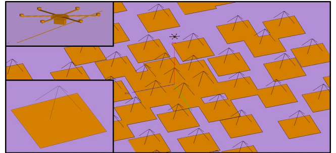
Fig. 1. Geometrical model of the LBA inner with the UAV. The UAV is shown at 5-m height from the array center for demonstration purpose. The insets on the left side show the UAV-mounted test source (top) and a single LBA (bottom).
