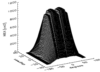
Fig. 11. Effective area of the three units for offsets of 35^\circ , giving a partial overlap of the fields of view of the three units.
