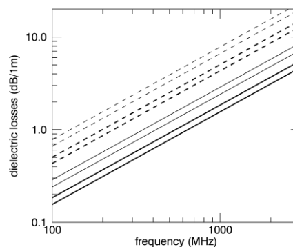
Figure 8 : Monostatic radar sensitivity: total dielectric losses in dB per meter with 40% porosity S-type asteroid permittivity (solid lines) ranges from 7.0 to 10.0 with a maximum loss tangent equal to 0.01. C-type asteroid permittivity (dashed lines) ranges from 5.9 to 8.2 with a maximum loss tangent equal to 0.03.
