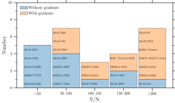
Fig. 7. Distribution of the S/N for the radio halos in the MGCLS grouped according to the presence or absence of radio surface brightness gradients.
