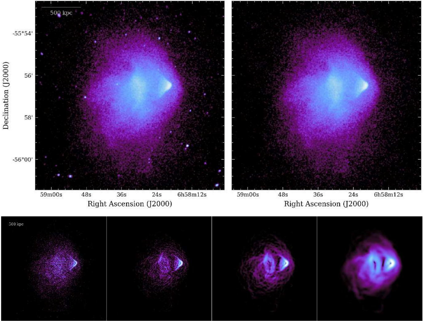
Fig. 2. X-ray images of the Bullet Cluster. Top panels: Chandra image in the 0.5–2.0 keV band of the thermal ICM with (left) and without (right) discrete sources. Bottom panels: GGM-filtered images obtained with \sigma = 1, 2, 4, 8 pixels (from left to right).
