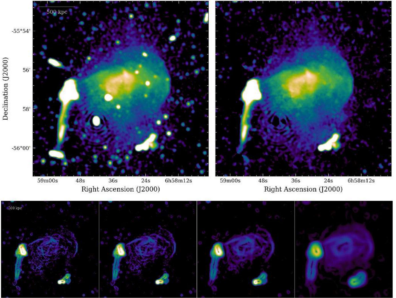
Fig. 1. Radio images of the Bullet Cluster. Top panels: MeerKAT image at 1.28 GHz of the radio halo with (left) and without (right) discrete sources. Bottom panels: GGM-filtered images obtained with \sigma = 1, 2, 4 , and 8 pixels (from left to right).
