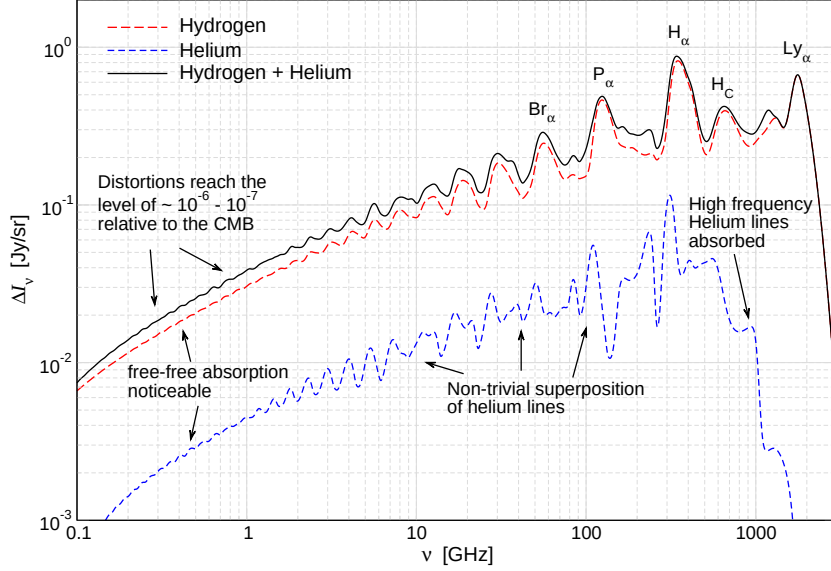
FIG. 7: The cosmological recombination radiation arising from the hydrogen and helium components. The helium distortion ( blue ) is the net accumulation of the Hel and Hell emission along with other effects (i.e. helium absorption and collisions). The spectral series of hydrogen have also been highlighted. The unique spectral shapes given by the CRR would provide us with a revolutionary new cosmological probe of the atomic physics in the early Universe.
