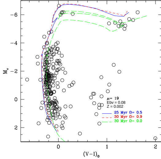
Figure 5. Color-magnitude diagram of NGC 330. The isochrone at 30 Myr is obtained from the Padova and TRIeste Stellar Evolution Code (PARSEC; Bressan et al. 2012 ; Marigo et al. 2017 ) (the green long-dashed line); the isochrones computed from rotating stellar models at 25 Myr with \omega = 0.5 \omega_c (blue line), and at 30 Myr with \omega = 0.9 \omega_c (red dashed line) are taken from Georgy et al. 2014 . The adopted values for the age, distance modulus, reddening, and metallicity are quoted in the figure.
