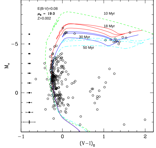
Figure 4. Color-magnitude diagram of the selected stars in NGC 330. The isochrones at 10 Myr, 18 Myr, 30 Myr and 50 Myr obtained from the Padova and TRIESTE Stellar Evolution Code (PARSEC; Bressan et al. 2012; Marigo et al. 2017) are overplotted with short green dashed, red solid and blue solid and cyan short-long lines, respectively. The best-fitting isochrones are 18 Myr and 30 Myr.
