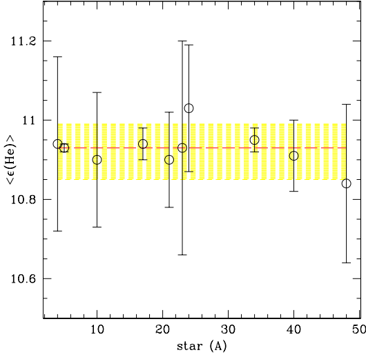
Figure 11. Mean value of the logarithmic He abundance for each target. Error bars are also shown. The red dashed line represents the average of these values, while the yellow shadow region shows the \pm 1\sigma level.
