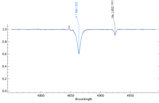
Figure 6. Best-fit of the H \beta and HeI lines (labelled) for the star A4.
