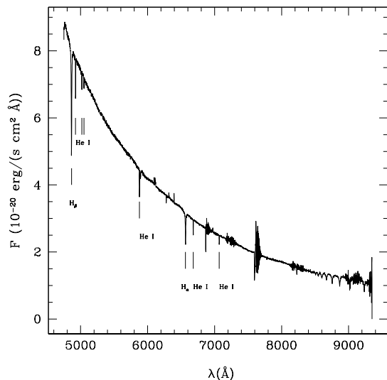
Figure 3. The entire spectrum of the B star A17 in NGC 330 obtained with MUSE@VLT.
