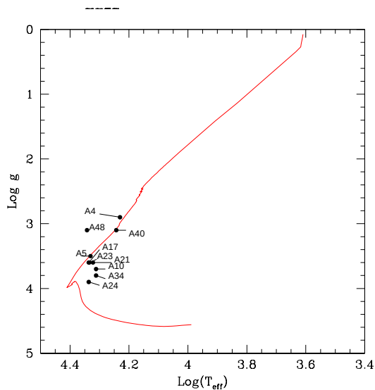
Figure 13. \log T_{\text{eff}} - \log g diagram for the stars analyzed spectroscopically by us with MUSE (black dots) considering stellar rotation. The Z = 0.002 SYCLIST isochrones of 30 Myr and \omega = 0.9\omega_c (Georgy et al. 2014) is reported with red solid line. We report also the name of the stars.
