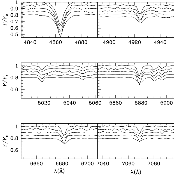
Figure 8. As for Fig. 7 but for the stars A23, A24, A34, A40, A48 (from top to bottom)
