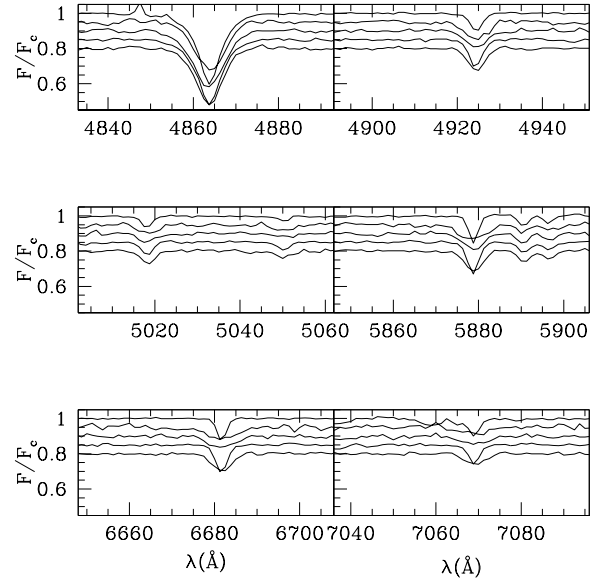
Figure 7. Each panel shows the region of the spectrum where the He features used in this work are located. The spectra are normalized but not red-shifted. In every panel the spectra of the stars A4, A5, A10, A17, A21 are plotted starting from the top and shifted of 0.05 in the y-axis for graphical reasons.
