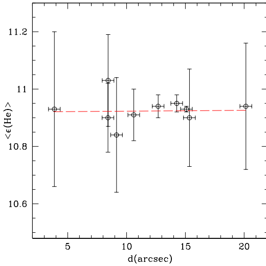
Figure 14. He abundance versus distance from the center of NGC 330 for our MUSE sample. Dashed line represents the linear best-fit to the data. The effective radius of NGC 330 is at 20'' .
