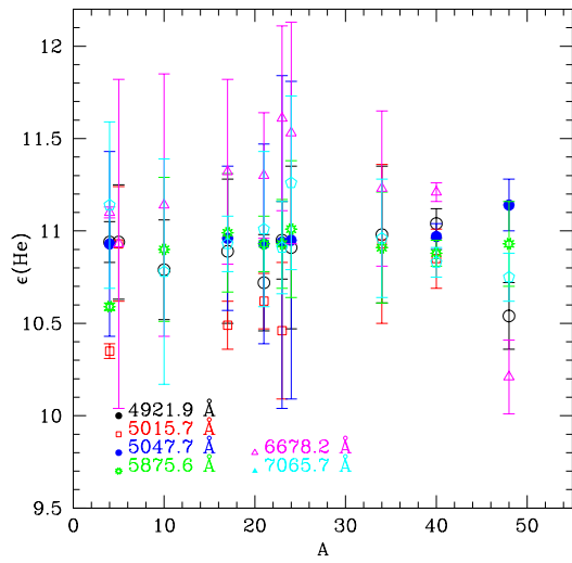
Figure 9. Logarithmic He abundance obtained for each helium line. Each symbol refers to different line. Uncertainties obtained by SME are also shown. x -axes reports the number of each star following the nomenclature by Robertson (1974).
