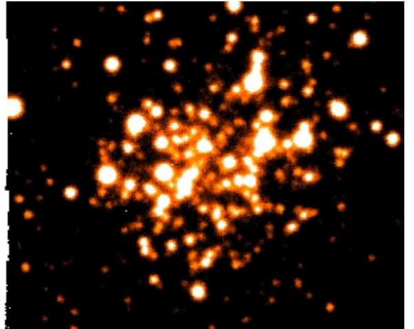
Figure 1. MUSE image of NGC330 at \lambda \sim 4800 Å. North is up and East is to the left. (For a color version of the figure see the electronic version of the paper).
