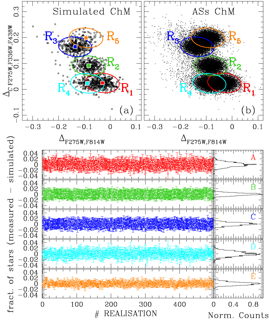
Figure 1. Panels (a) and (b) show the simulated and the ASs ChMs. The coloured ellipses are the regions R_i within our analysis has been performed. Left-hand bottom panels shows the difference between the measured and the expected fraction of stars at each of the 500 realisations of the simulated ChM. As shown in the right-hand bottom panels, the distributions of these differences is centred on zero.
