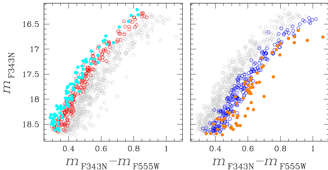
Figure 8. The m_{F343N} vs. m_{F343N} - m_{F555W} CMDs of RGB stars in M15. Population A and D stars are coloured red and cyan. Blue and orange colours indicate populations C and E, respectively.
