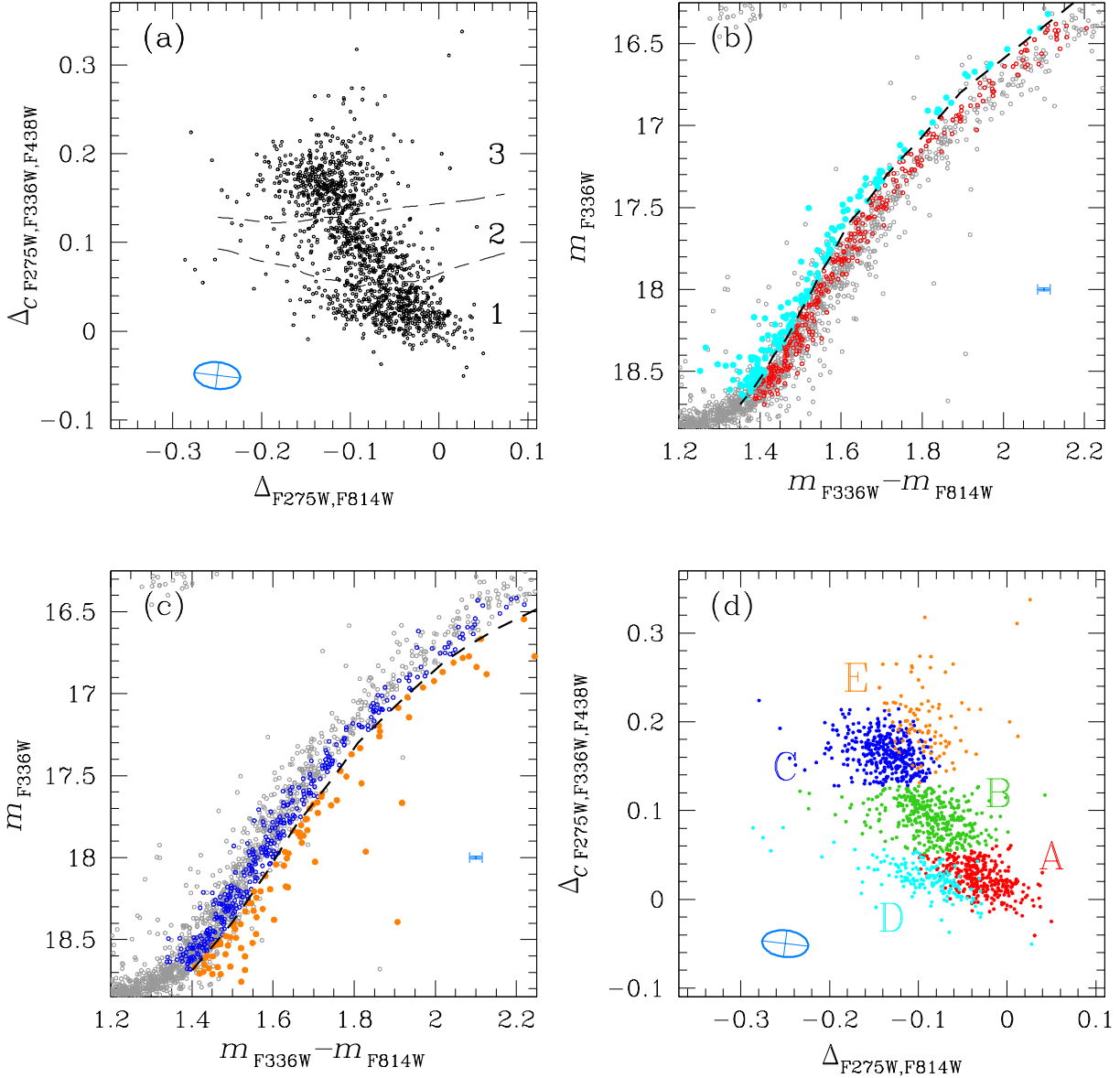
Figure 6. Procedure adopted to identify the different populations hosted by M 15. The dashed lines overimposed on the ChM shown in the panel (a) are used to identify the three groups of RGB-1, RGB-2 and RGB-3 stars. Panels (b) and (c) show the m_{F336W} vs. m_{F336W} - m_{F814W} CMD of RGB stars. The dashed lines plotted in the panels (b) and (c) are used to separate the two sub-populations A and D of the RGB-1 and the sub-populations C and E of the RGB-3, respectively. In panel (d) we use red, green, blue, cyan, and orange colours to represent stars in the populations A, B, C, D, and E, respectively, in the ChM. See text for details.
