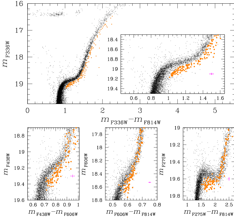
Figure 10. Top panel: m_{F336W} versus m_{F336W} - m_{F814W} CMD of M15, with the POPE coloured in orange. The inset shows a zoom-in around the SGB region. The faint SGB, possibly associated with POPE, is highlighted in orange. Bottom panels: m_{F438W} versus m_{F438W} - m_{F606W} (left), m_{F606W} versus m_{F606W} - m_{F814W} (middle), and m_{F275W} versus m_{F275W} - m_{F814W} (right) CMDs around the SGB region. The faint SGB stars selected in the top panel are coloured in orange in these CMDs as well. The magenta crosses show the photometric errors at the SGB level.
