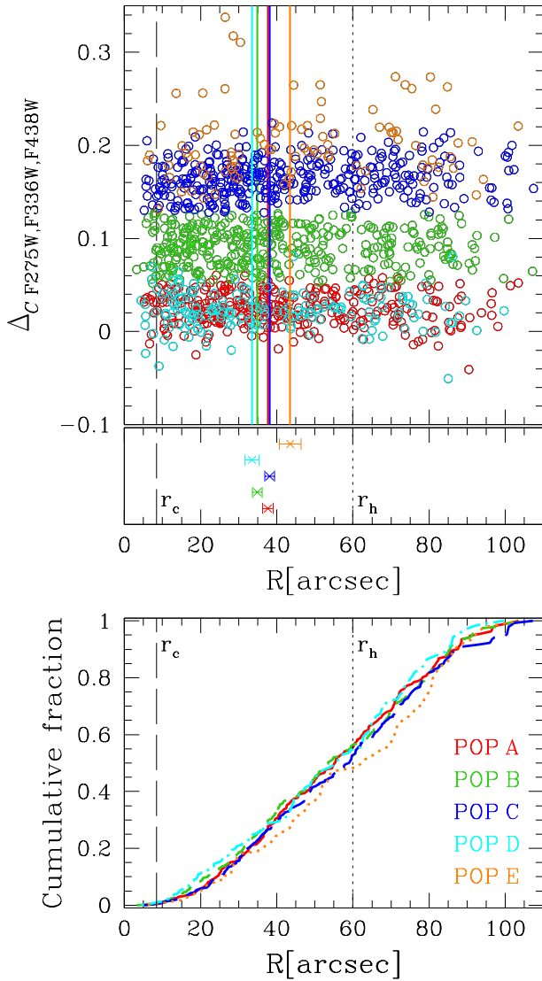
Figure 13. Top panel shows the pseudo-colour \Delta_{CF275W,F336W,F438W} as a function of the distance from the centre of M15. The red, green, blue, cyan, and orange vertical lines are the median radial coordinates of POP A, POP B, POP C, POP D, and POPE, respectively. The median radial coordinates of the different populations are also reported in the middle panel, with the error-bars as shown. Bottom panel shows the cumulative radial distributions for each population. All populations share the same radial trend. Dashed and dotted vertical lines are the core (8.4 arcsec) and the half-light (60 arcsec) radii, as reported in Harris (1996, updated to December 2010) .
