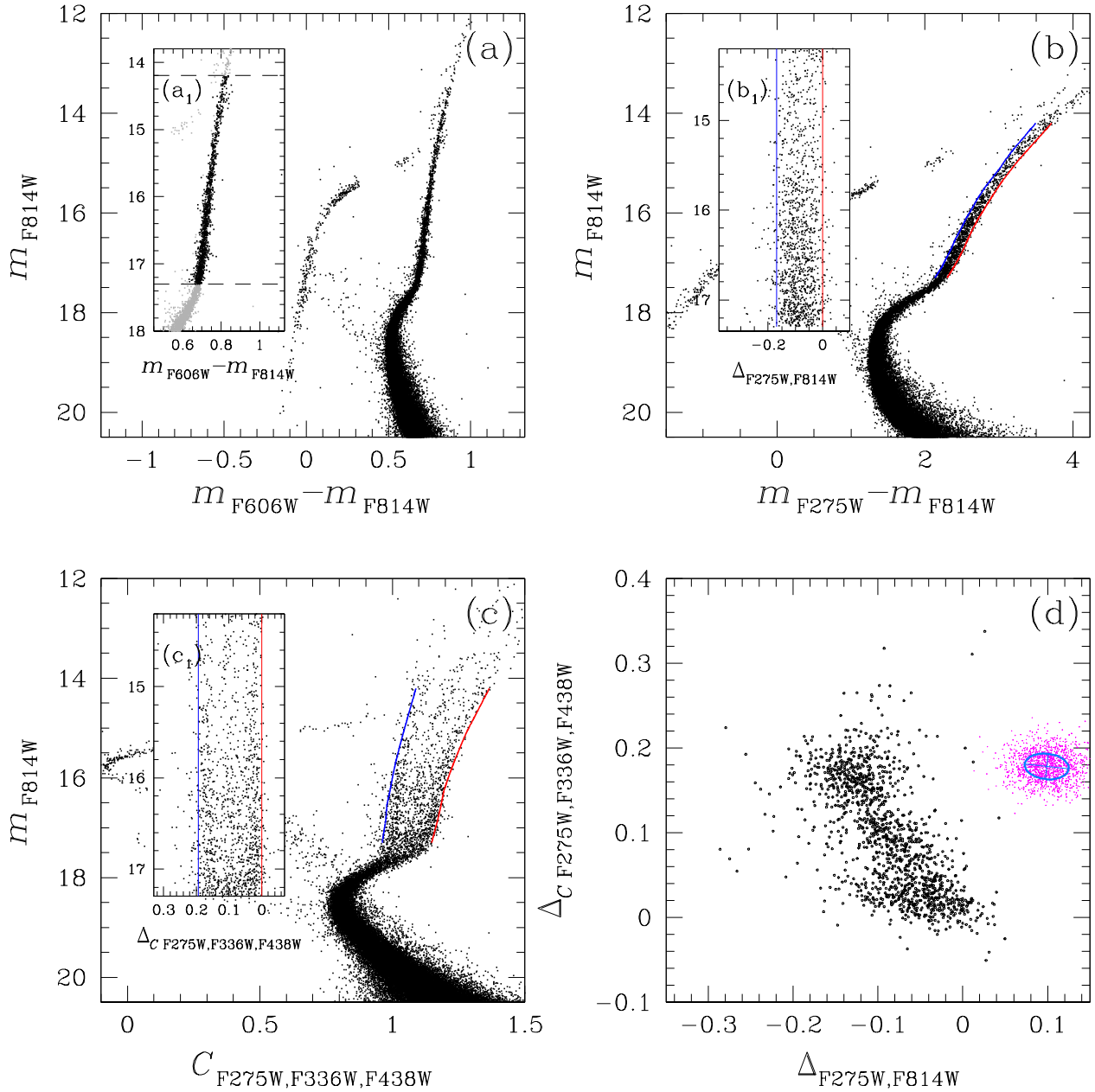
Figure 5. This figure illustrates the procedure adopted to derive the \Delta_{CF275W,F336W,F438W} versus \Delta_{F275W,F814W} ChM of RGB stars in M15. Panel (a): the m_{F814W} versus m_{F606W} - m_{F814W} CMD of M15. The inset panel (a 1 ) shows a zoom-in on the RGB region: grey and black points represent all the well-measured stars and the selected RGB stars, respectively. Panels (b) and (c): the m_{F814W} versus m_{F275W} - m_{F814W} and the m_{F814W} versus C_{F275W,F336W,F438W} CMDs of M15, respectively. The blue and red lines are the fiducials used to verticalize the RGB (inset panels (b 1 ) and (c 1 )), and correspond to the 4th and 96 th percentile of the RGB colour distribution. Panel (d): \Delta_C F275W,F336W,F438W versus \Delta_{F275W,F814W} ChM, obtained as explained in the text. The points in magenta are the distribution of the observational errors; the azure ellipse include the 68.27 per cent of the points.
