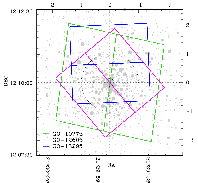
Figure 1. Footprint of the HST ACS and WFC3 observations used in this analysis. The inner circle is the core radius ( r_c = 0.14 arcmin), the outer circle is the half-light radius ( r_h = 1.0 arcmin; Harris 1996, updated to December 2010).
