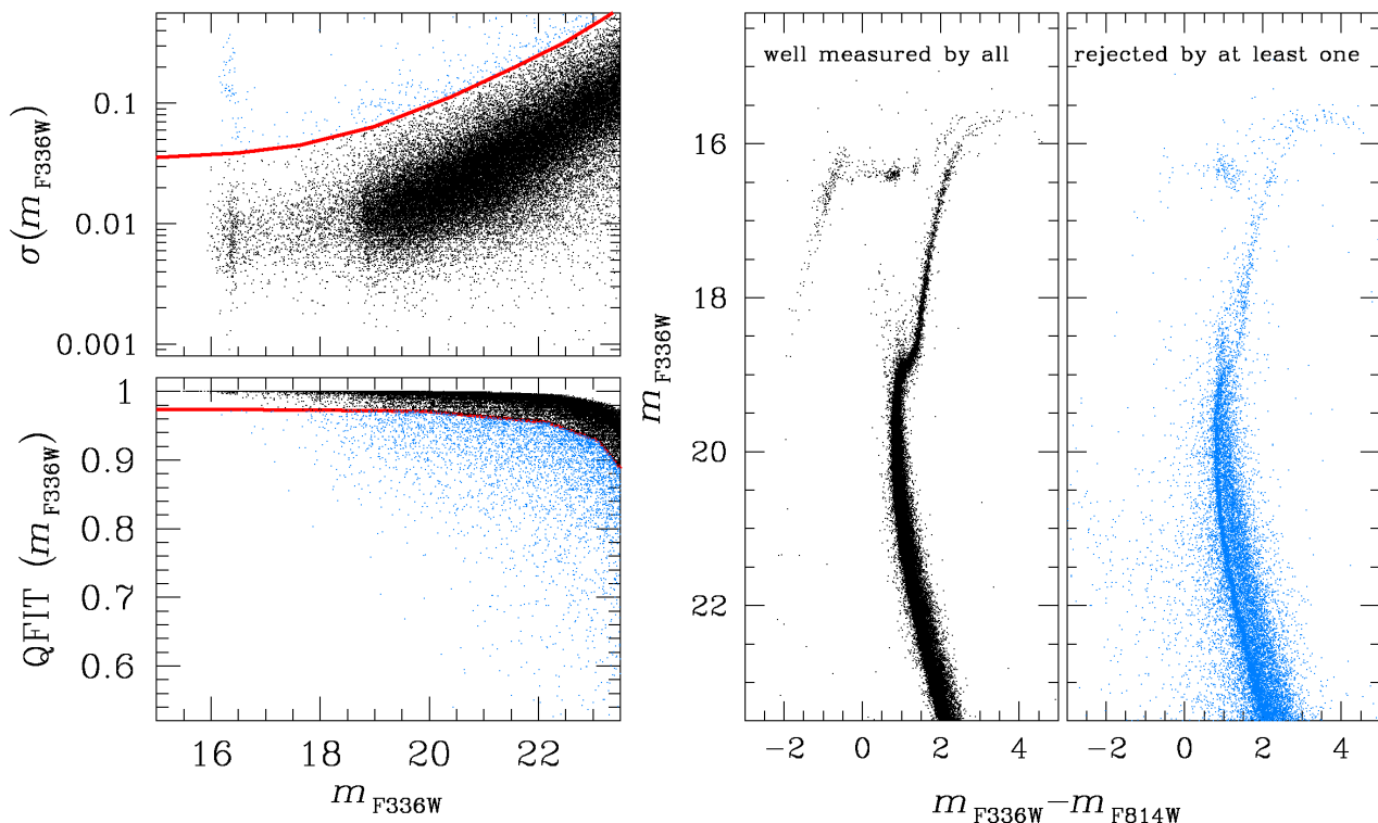
Figure 2. Selection of well measured stars based on photometric errors (top-left panel) and QFIT (bottom-left panel), for the filter F336W: in black the stars that satisfy the selection criteria, in azure the rejected stars. Similar selections have been performed for the other filters. The CMD in the central panel shows the stars that passed the selections in the F336W and F814W filters; the right panel shows the CMD of the stars rejected by at least one of selection cuts.
