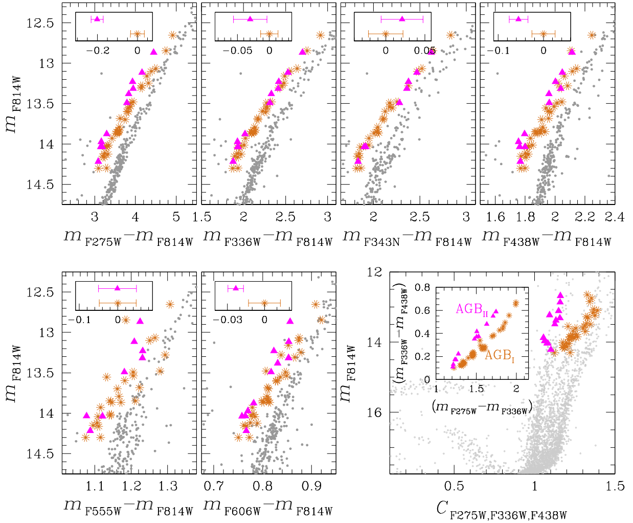
Figure 11. Analysis of AGB stars. Top-panels and first two bottom panels show the m_{F814W} versus m_X - m_{F814W} CMDs, with X=F275W, F336W, F343N, F438W, F555W and F606W ; the inset panels show the average colour difference between AGB_I and AGB_{II} sequences. The right-hand bottom panel shows the m_{F814W} versus C_{F275W,F336W,F438W} pseudo-CMD for all the stars (grey points) and for AGB stars (coloured points). Inset panel is the m_{F336W} - m_{F438W} versus m_{F275W} - m_{F336W} two-colour diagram of AGB stars. In all the diagrams, brown starred dots and magenta triangles represent the AGB_I and AGB_{II} stars, respectively.
