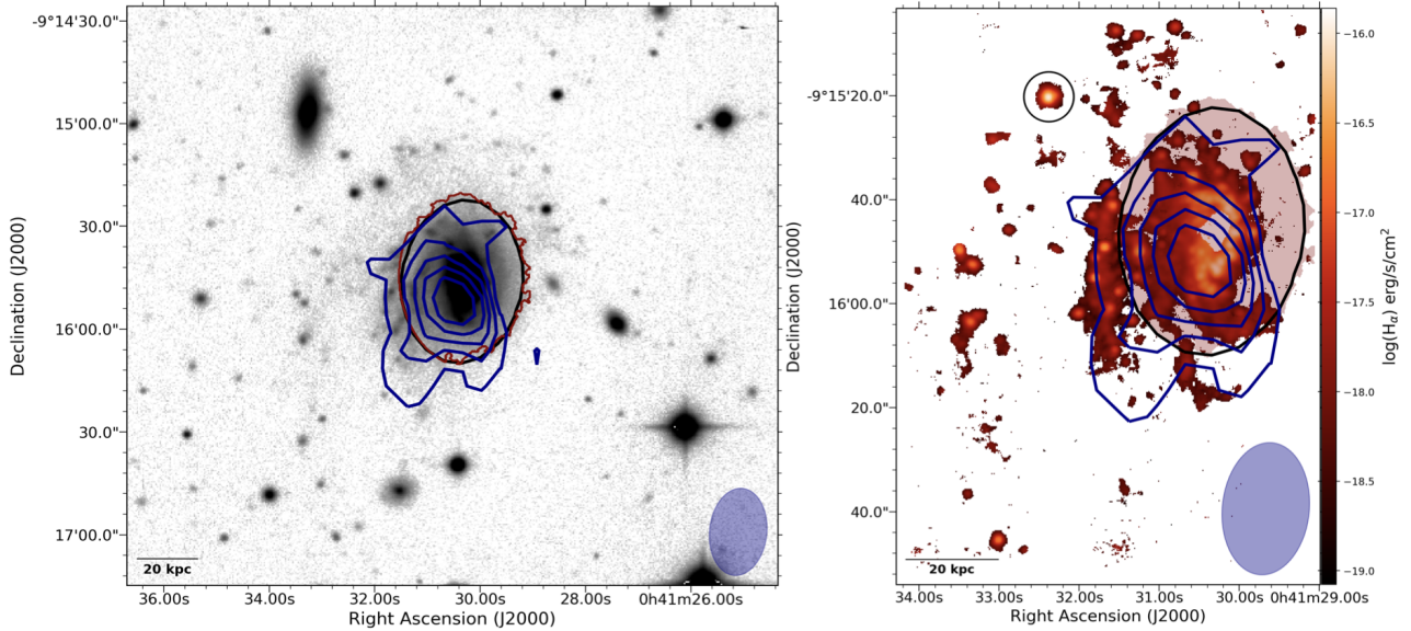
Fig. 2. Left panel: VLA HI column density contours overlaid on the V-band image of JO201 from WINGS. Contour levels are drawn at column densities of 4, 8, 12, \dots \times 10^{19} \text{ atoms cm}^{-2} . The FWHM beam size of 16'' \times 25'' is indicated by the blue ellipse. The red contours represent the stellar disc and the black contour is the HI disc (see text for a definition). Right panel: H \alpha emission with HI column density contours (same levels as the left panel) overlaid. The red opaque patch is the stellar disc and the black contour is the HI disc. The black circle is the region over which we estimate the HI flux density as described in the text.
