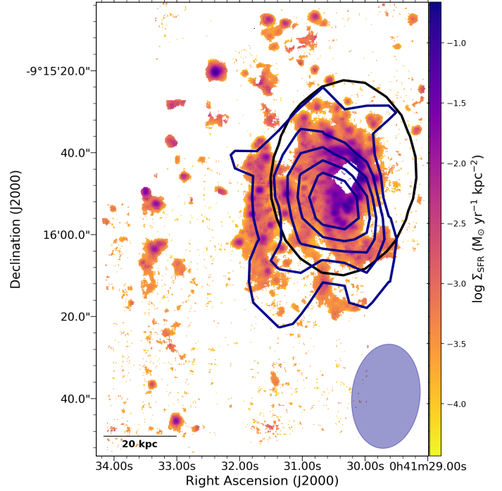
Fig. 4. Star formation rate density map (Bellhouse et al. 2019) with HI emission contours overlaid. The contours are at HI column density levels of 4, 8, 12, \dots \times 10^{19} \text{ atoms cm}^{-2} . The FWHM beam size of 25'' \times 16'' is shown by the blue ellipse.
