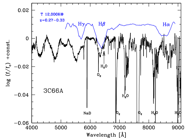
Figure 7. The linearized 3C 66A spectrum, compared with a BLUESED synthetic spectrum of a stellar model atmosphere with T = 12000 K shifted within the range 0.27 < z < 0.33 (blue line). The Balmer sequence of the H\gamma , H\beta and H\alpha absorption lines might be recognized to match the blazar spectrum. See the text for a discussion.
