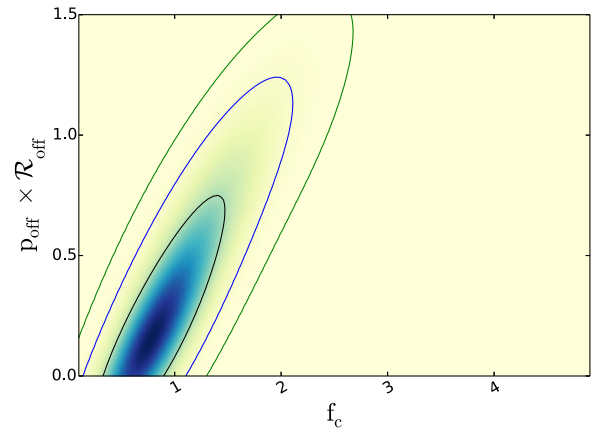
Figure 11. 2D posterior distribution of the average projected offset ( p_{\text{off}} \times \mathcal{R}_{\text{off}} ) and the normalization of the concentration–halo mass relation f_c . The contours indicate the 68, 95, and 99 per cent confidence region.
